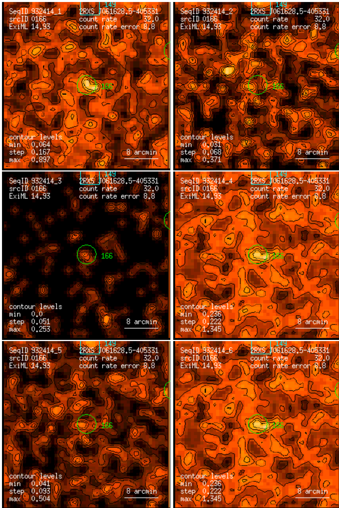
Figure 166: RASS 932414: detection 0166: band rate images, Gaussian filter: (1) PSPC channels 11 – 41, (2) 52 – 90, (3) 91 – 201, (4) 11 – 235, (5) 52 – 201, (6) 11 – 201. Broad band rates in counts/ks. Band rate contour levels in counts/ks/arcmin 2 .
