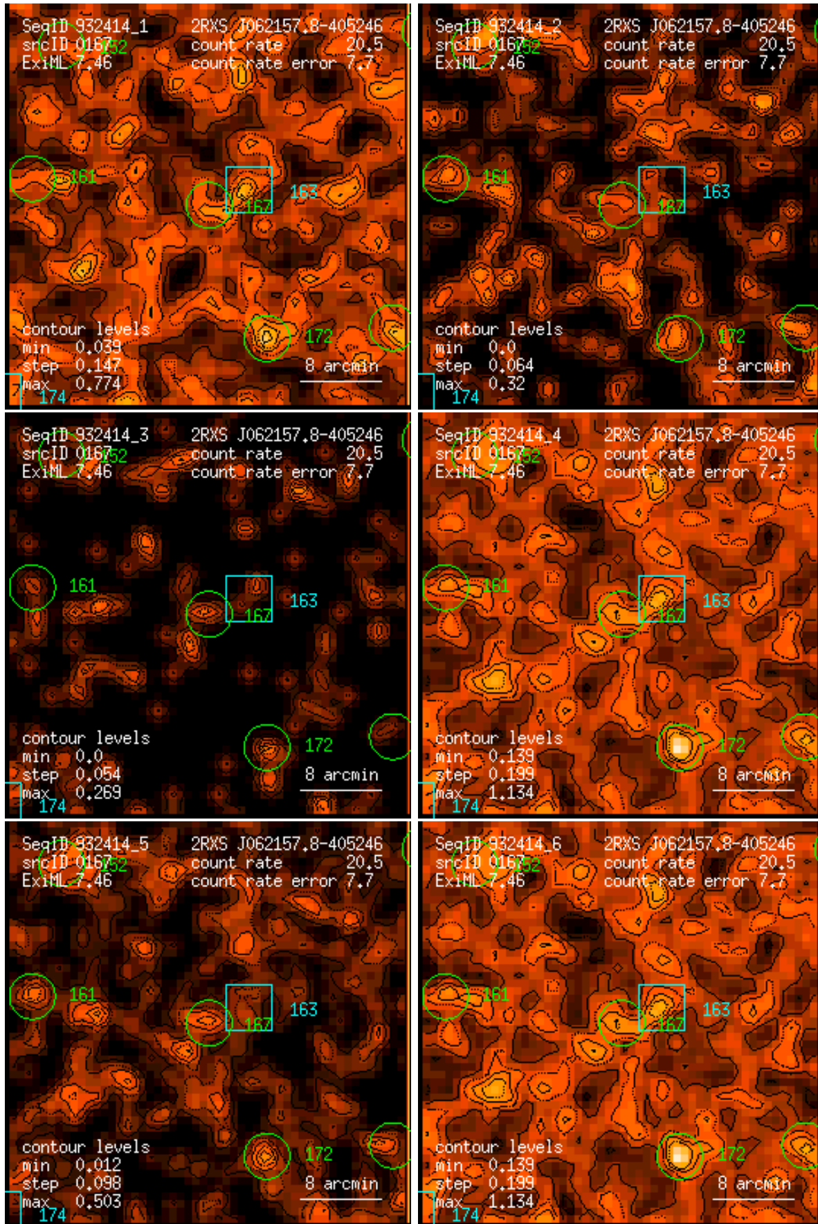
Figure 167: RASS 932414: detection 0167: band rate images, Gaussian filter: (1) PSPC channels 11 – 41, (2) 52 – 90, (3) 91 – 201, (4) 11 – 235, (5) 52 – 201, (6) 11 – 201. Broad band rates in counts/ks. Band rate contour levels in counts/ks/arcmin 2 .
