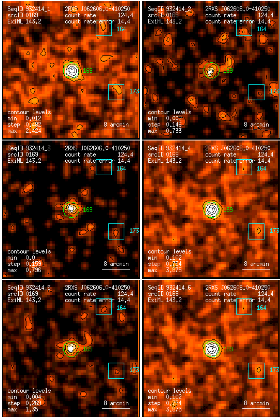
Figure 169: RASS 932414: detection 0169: band rate images, Gaussian filter: (1) PSPC channels 11 – 41, (2) 52 – 90, (3) 91 – 201, (4) 11 – 235, (5) 52 – 201, (6) 11 – 201. Broad band rates in counts/ks. Band rate contour levels in counts/ks/arcmin 2 .
