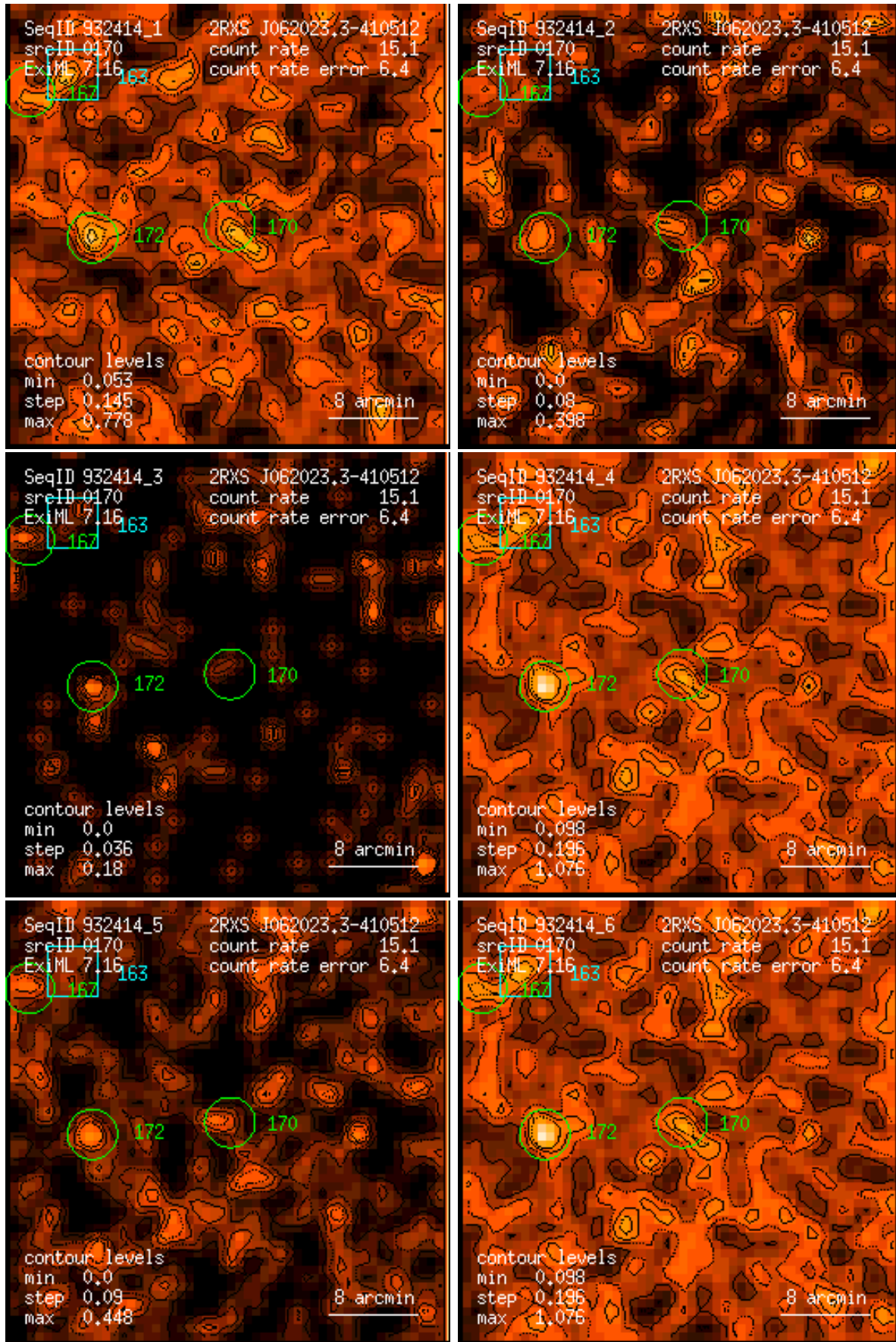
Figure 170: RASS 932414: detection 0170: band rate images, Gaussian filter: (1) PSPC channels 11 – 41, (2) 52 – 90, (3) 91 – 201, (4) 11 – 235, (5) 52 – 201, (6) 11 – 201. Broad band rates in counts/ks. Band rate contour levels in counts/ks/arcmin 2 .
