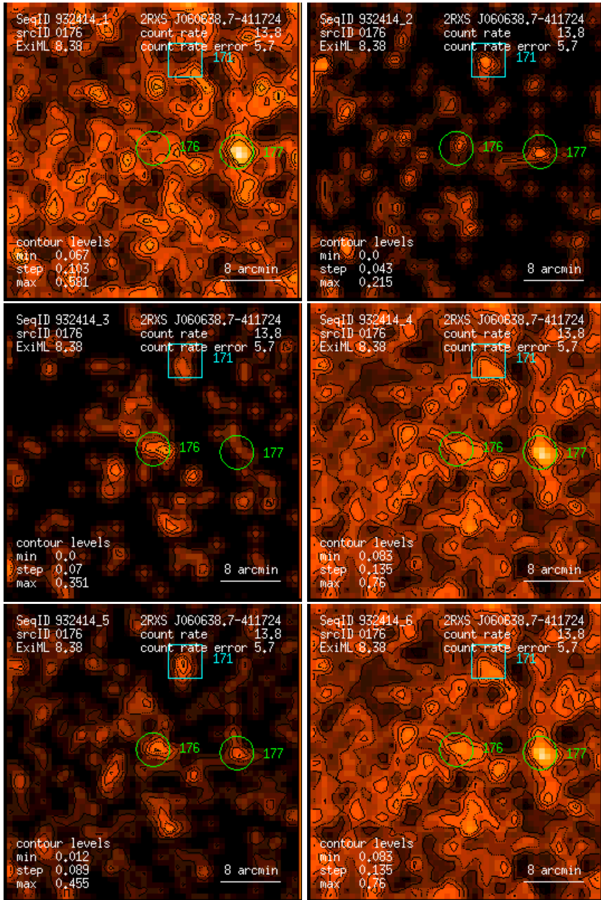
Figure 176: RASS 932414: detection 0176: band rate images, Gaussian filter: (1) PSPC channels 11 – 41, (2) 52 – 90, (3) 91 – 201, (4) 11 – 235, (5) 52 – 201, (6) 11 – 201. Broad band rates in counts/ks. Band rate contour levels in counts/ks/arcmin 2 .
