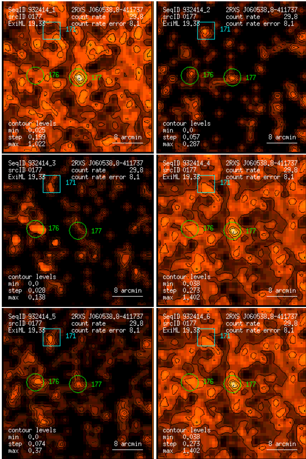
Figure 177: RASS 932414: detection 0177: band rate images, Gaussian filter: (1) PSPC channels 11 – 41, (2) 52 – 90, (3) 91 – 201, (4) 11 – 235, (5) 52 – 201, (6) 11 – 201. Broad band rates in counts/ks. Band rate contour levels in counts/ks/arcmin 2 .
