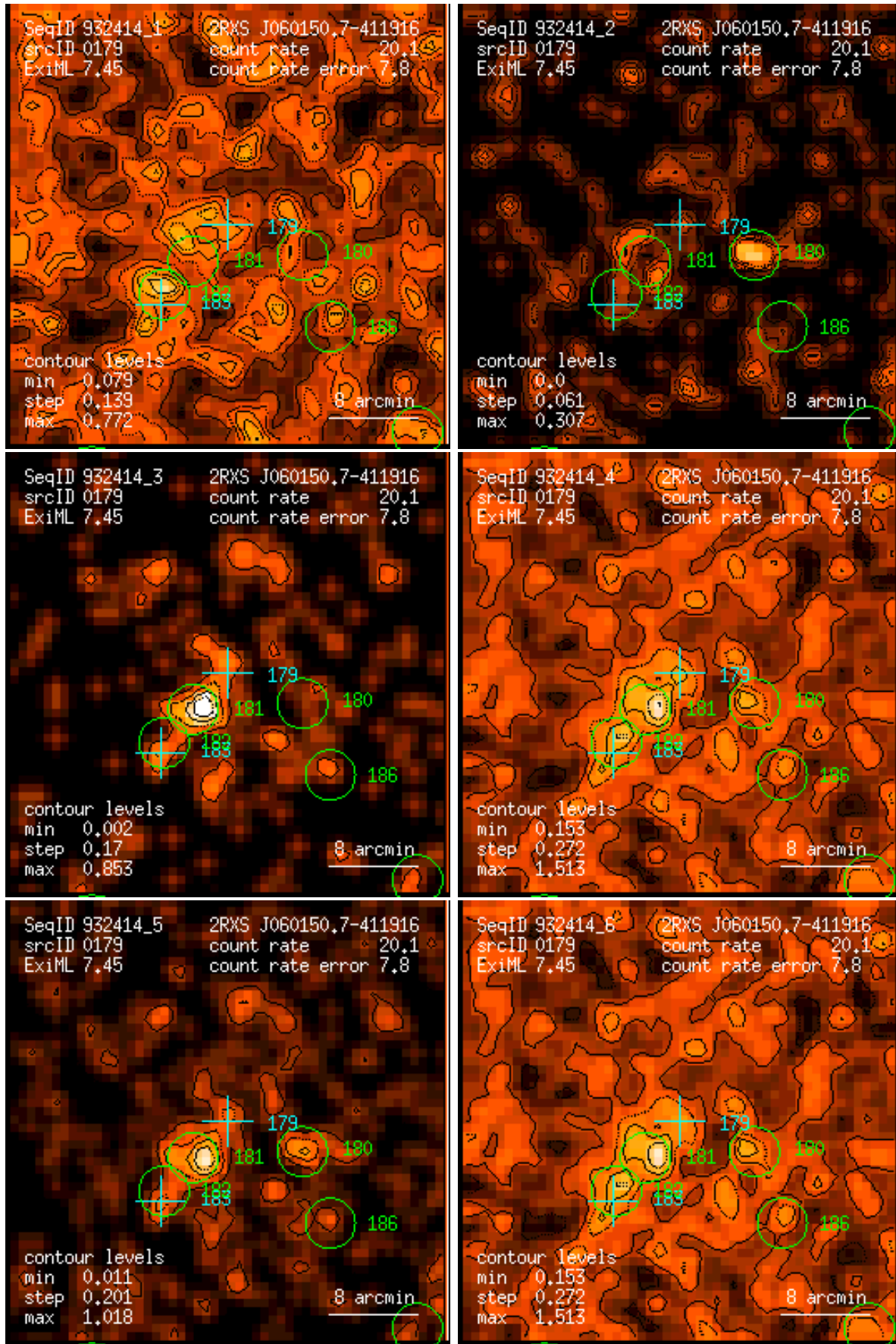
Figure 179: RASS 932414: detection 0179: band rate images, Gaussian filter: (1) PSPC channels 11 – 41, (2) 52 – 90, (3) 91 – 201, (4) 11 – 235, (5) 52 – 201, (6) 11 – 201. Broad band rates in counts/ks. Band rate contour levels in counts/ks/arcmin 2 .
