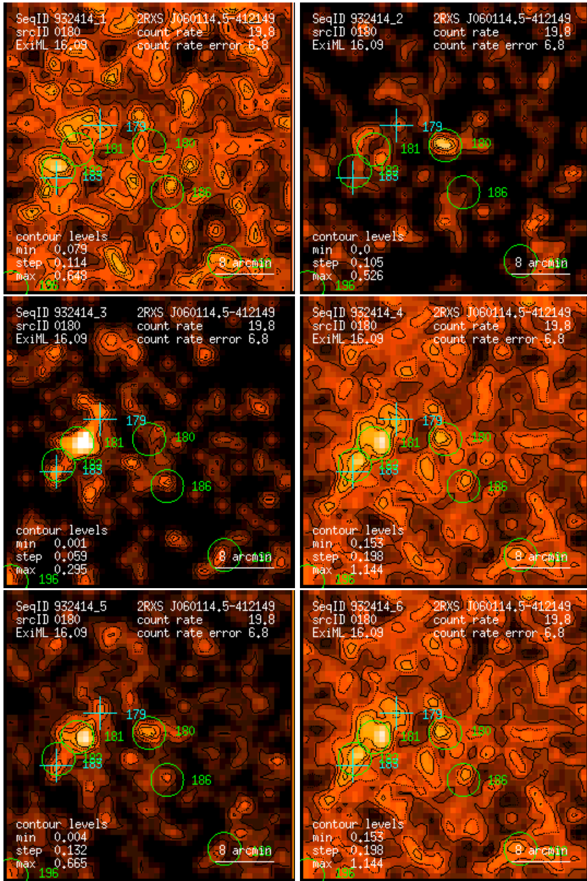
Figure 180: RASS 932414: detection 0180: band rate images, Gaussian filter: (1) PSPC channels 11 – 41, (2) 52 – 90, (3) 91 – 201, (4) 11 – 235, (5) 52 – 201, (6) 11 – 201. Broad band rates in counts/ks. Band rate contour levels in counts/ks/arcmin 2 .
