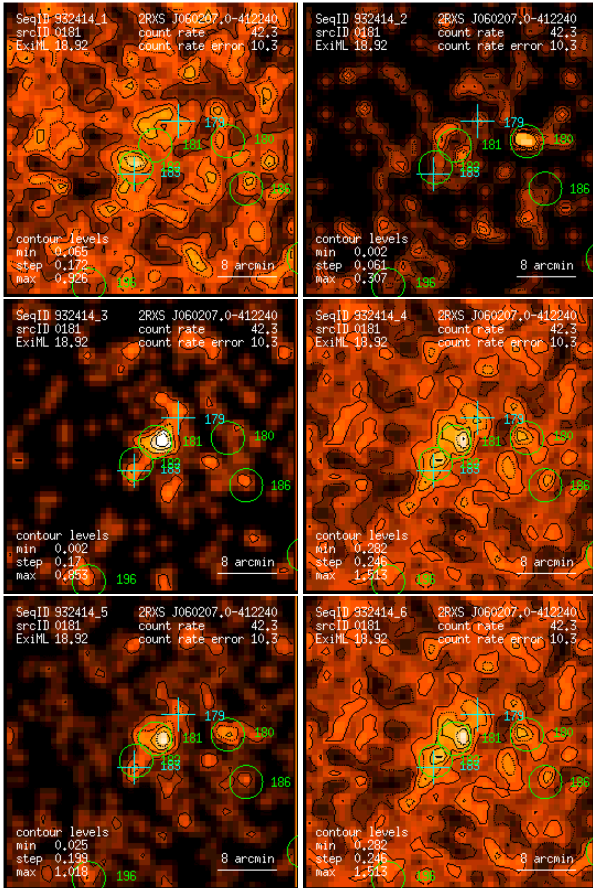
Figure 181: RASS 932414: detection 0181: band rate images, Gaussian filter: (1) PSPC channels 11 – 41, (2) 52 – 90, (3) 91 – 201, (4) 11 – 235, (5) 52 – 201, (6) 11 – 201. Broad band rates in counts/ks. Band rate contour levels in counts/ks/arcmin 2 .
