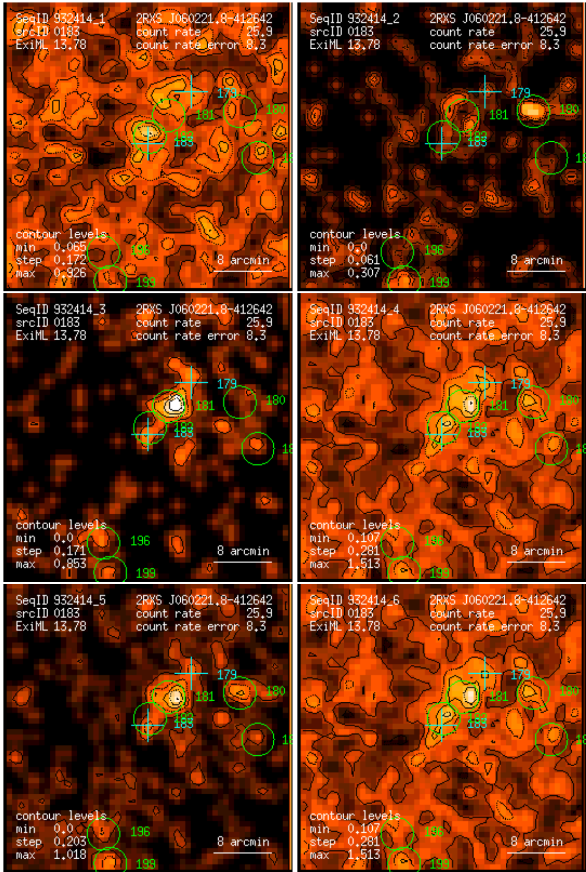
Figure 183: RASS 932414: detection 0183: band rate images, Gaussian filter: (1) PSPC channels 11 – 41, (2) 52 – 90, (3) 91 – 201, (4) 11 – 235, (5) 52 – 201, (6) 11 – 201. Broad band rates in counts/ks. Band rate contour levels in counts/ks/arcmin 2 .
