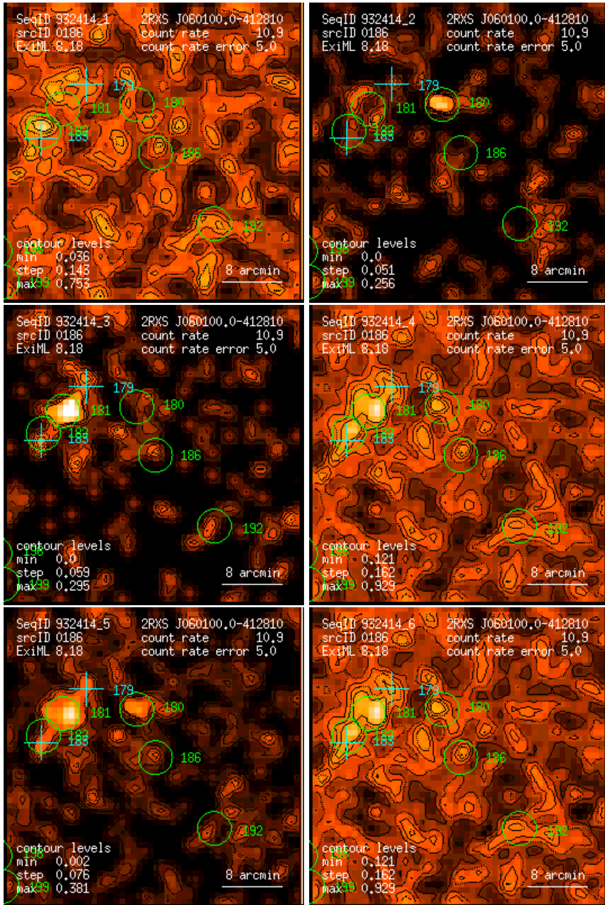
Figure 186: RASS 932414: detection 0186: band rate images, Gaussian filter: (1) PSPC channels 11 – 41, (2) 52 – 90, (3) 91 – 201, (4) 11 – 235, (5) 52 – 201, (6) 11 – 201. Broad band rates in counts/ks. Band rate contour levels in counts/ks/arcmin 2 .
