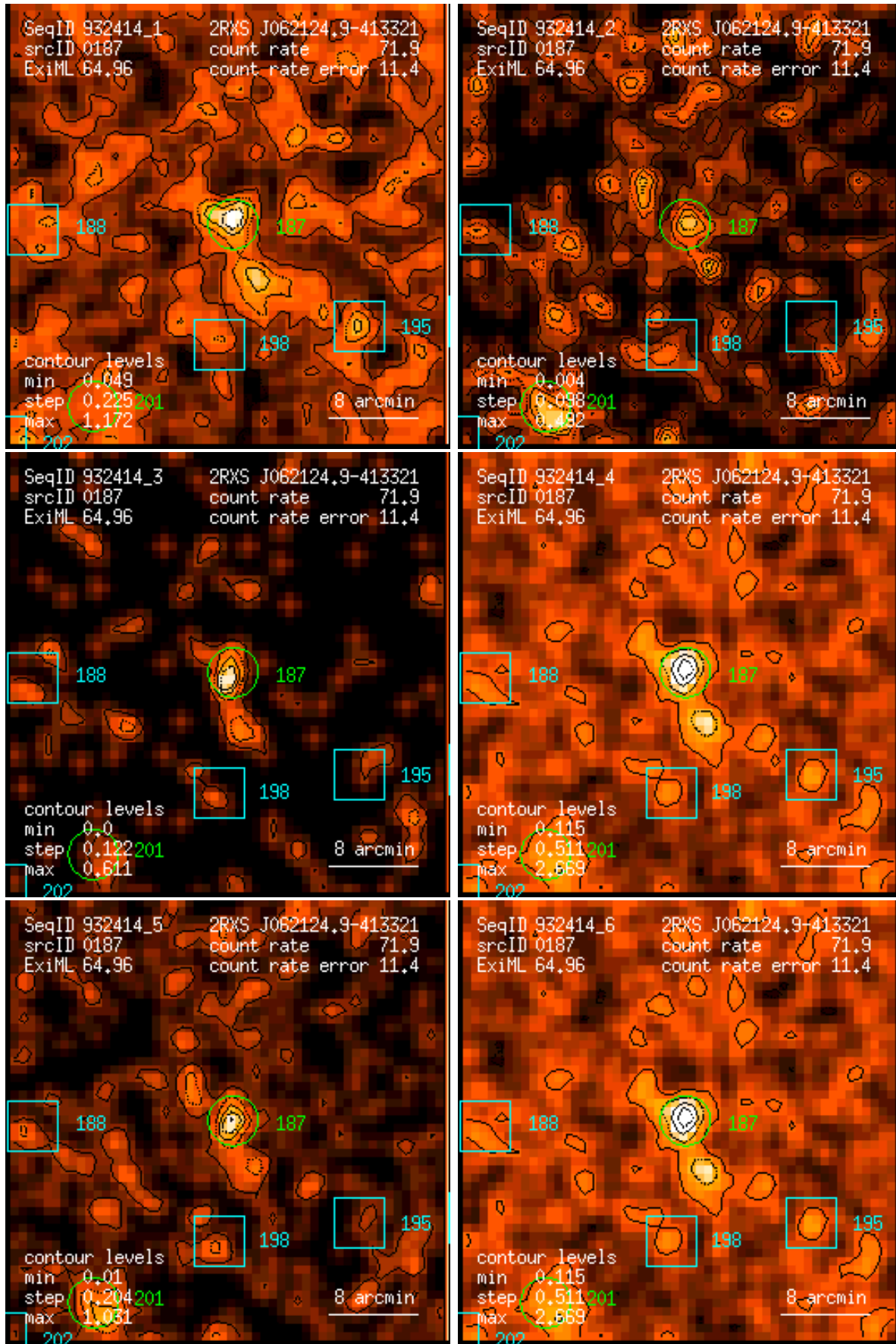
Figure 187: RASS 932414: detection 0187: band rate images, Gaussian filter: (1) PSPC channels 11 – 41, (2) 52 – 90, (3) 91 – 201, (4) 11 – 235, (5) 52 – 201, (6) 11 – 201. Broad band rates in counts/ks. Band rate contour levels in counts/ks/arcmin 2 .
