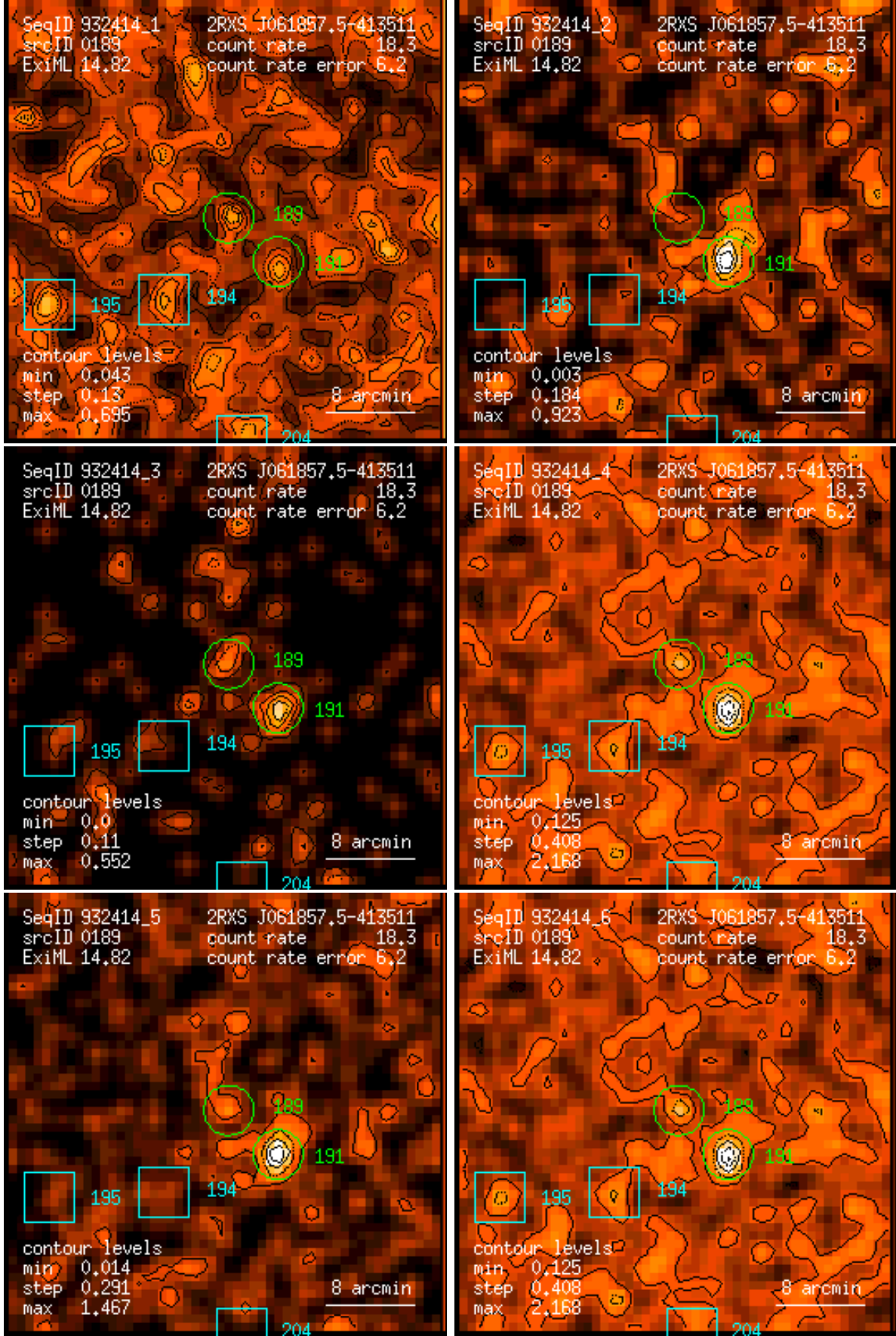
Figure 189: RASS 932414: detection 0189: band rate images, Gaussian filter: (1) PSPC channels 11 – 41, (2) 52 – 90, (3) 91 – 201, (4) 11 – 235, (5) 52 – 201, (6) 11 – 201. Broad band rates in counts/ks. Band rate contour levels in counts/ks/arcmin 2 .
