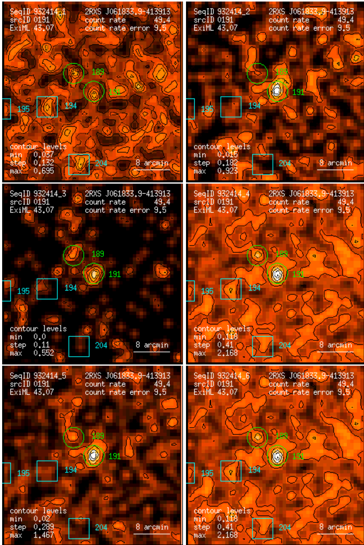
Figure 191: RASS 932414: detection 0191: band rate images, Gaussian filter: (1) PSPC channels 11 – 41, (2) 52 – 90, (3) 91 – 201, (4) 11 – 235, (5) 52 – 201, (6) 11 – 201. Broad band rates in counts/ks. Band rate contour levels in counts/ks/arcmin 2 .
