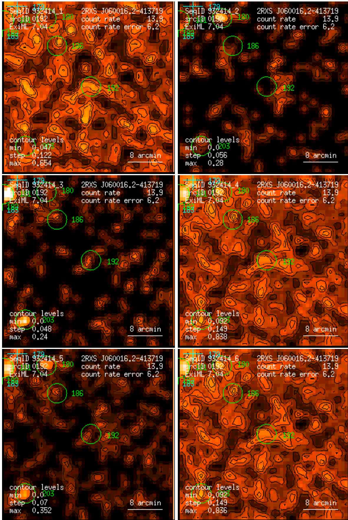
Figure 192: RASS 932414: detection 0192: band rate images, Gaussian filter: (1) PSPC channels 11 – 41, (2) 52 – 90, (3) 91 – 201, (4) 11 – 235, (5) 52 – 201, (6) 11 – 201. Broad band rates in counts/ks. Band rate contour levels in counts/ks/arcmin 2 .
