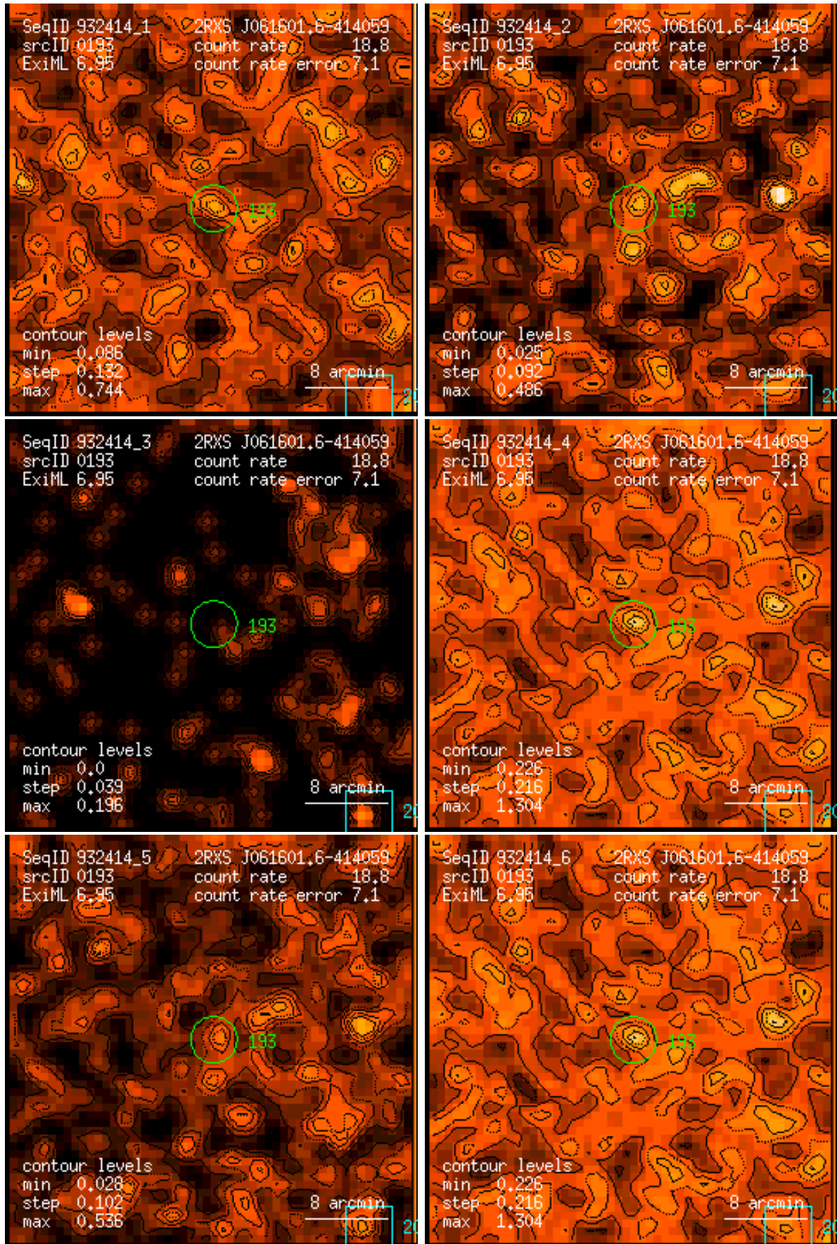
Figure 193: RASS 932414: detection 0193: band rate images, Gaussian filter: (1) PSPC channels 11 – 41, (2) 52 – 90, (3) 91 – 201, (4) 11 – 235, (5) 52 – 201, (6) 11 – 201. Broad band rates in counts/ks. Band rate contour levels in counts/ks/arcmin 2 .
