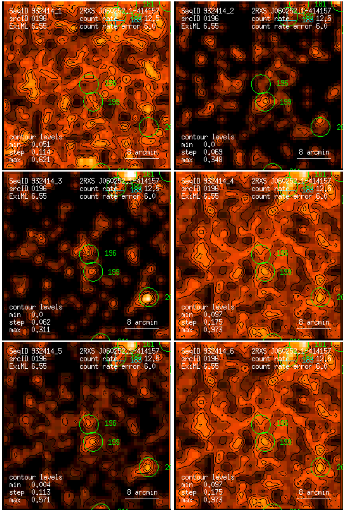
Figure 196: RASS 932414: detection 0196: band rate images, Gaussian filter: (1) PSPPC channels 11 – 41, (2) 52 – 90, (3) 91 – 201, (4) 11 – 235, (5) 52 – 201, (6) 11 – 201. Broad band rates in counts/ks. Band rate contour levels in counts/ks/arcmin 2 .
