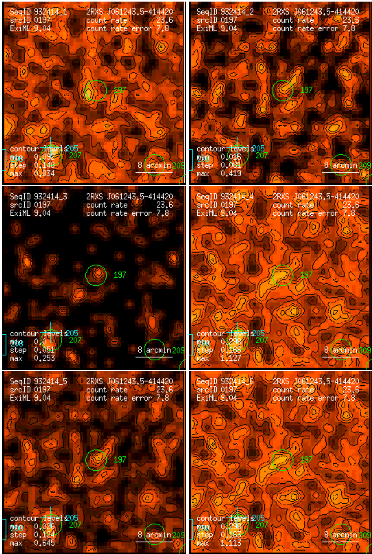
Figure 197: RASS 932414: detection 0197: band rate images, Gaussian filter: (1) PSPC channels 11 – 41, (2) 52 – 90, (3) 91 – 201, (4) 11 – 235, (5) 52 – 201, (6) 11 – 201. Broad band rates in counts/ks. Band rate contour levels in counts/ks/arcmin 2 .
