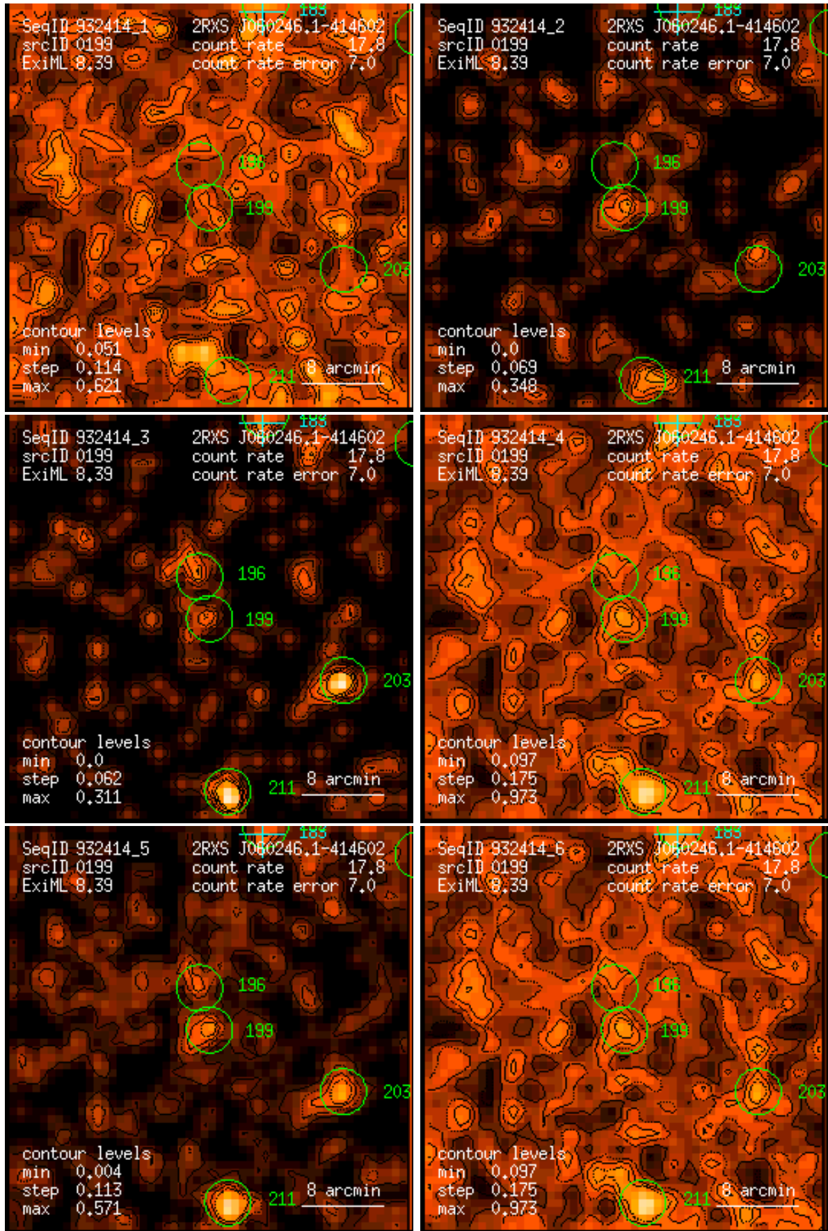
Figure 199: RASS 932414: detection 0199: band rate images, Gaussian filter: (1) PSPC channels 11 – 41, (2) 52 – 90, (3) 91 – 201, (4) 11 – 235, (5) 52 – 201, (6) 11 – 201. Broad band rates in counts/ks. Band rate contour levels in counts/ks/arcmin 2 .
