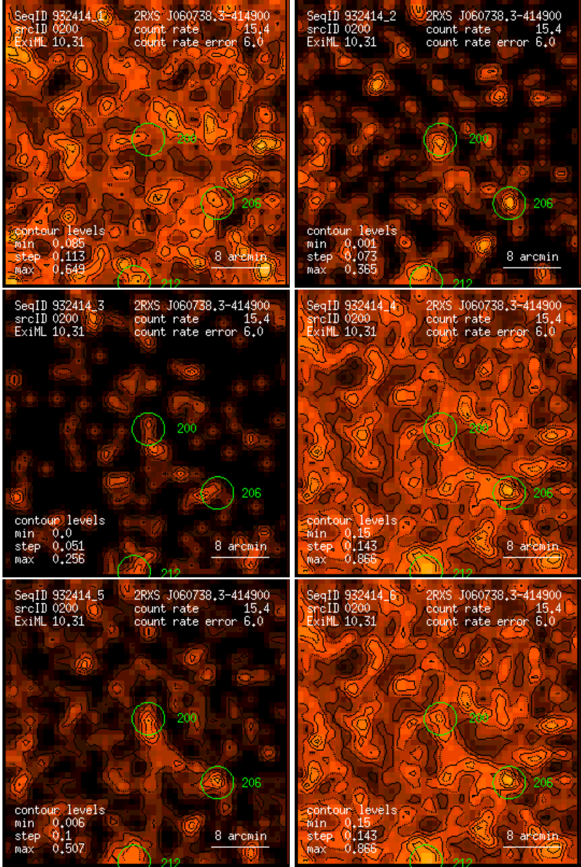
Figure 200: RASS 932414: detection 0200: band rate images, Gaussian filter: (1) PSPC channels 11 – 41, (2) 52 – 90, (3) 91 – 201, (4) 11 – 235, (5) 52 – 201, (6) 11 – 201. Broad band rates in counts/ks. Band rate contour levels in counts/ks/arcmin 2 .
