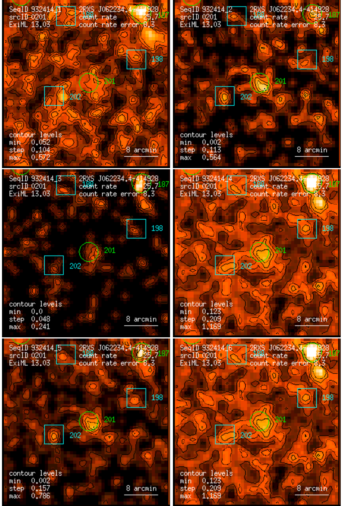
Figure 201: RASS 932414: detection 0201: band rate images, Gaussian filter: (1) PSPC channels 11 – 41, (2) 52 – 90, (3) 91 – 201, (4) 11 – 235, (5) 52 – 201, (6) 11 – 201. Broad band rates in counts/ks. Band rate contour levels in counts/ks/arcmin 2 .
