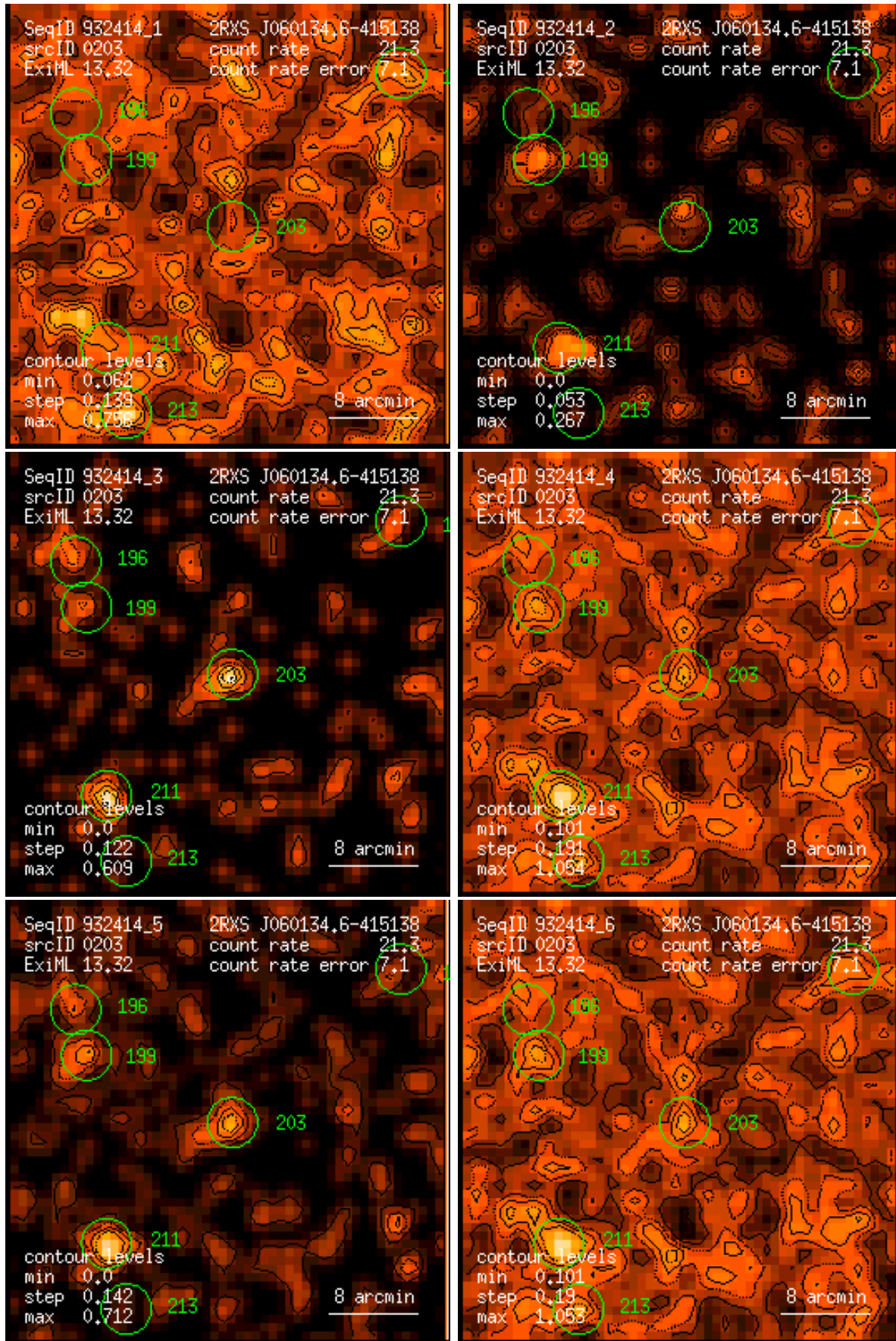
Figure 203: RASS 932414: detection 0203: band rate images, Gaussian filter: (1) PSPC channels 11 – 41, (2) 52 – 90, (3) 91 – 201, (4) 11 – 235, (5) 52 – 201, (6) 11 – 201. Broad band rates in counts/ks. Band rate contour levels in counts/ks/arcmin 2 .
