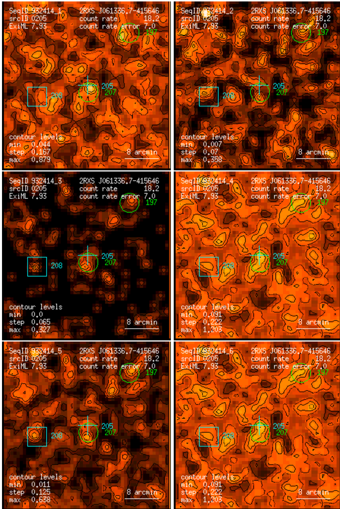
Figure 205: RASS 932414: detection 0205: band rate images, Gaussian filter: (1) PSPC channels 11 – 41, (2) 52 – 90, (3) 91 – 201, (4) 11 – 235, (5) 52 – 201, (6) 11 – 201. Broad band rates in counts/ks. Band rate contour levels in counts/ks/arcmin 2 .
