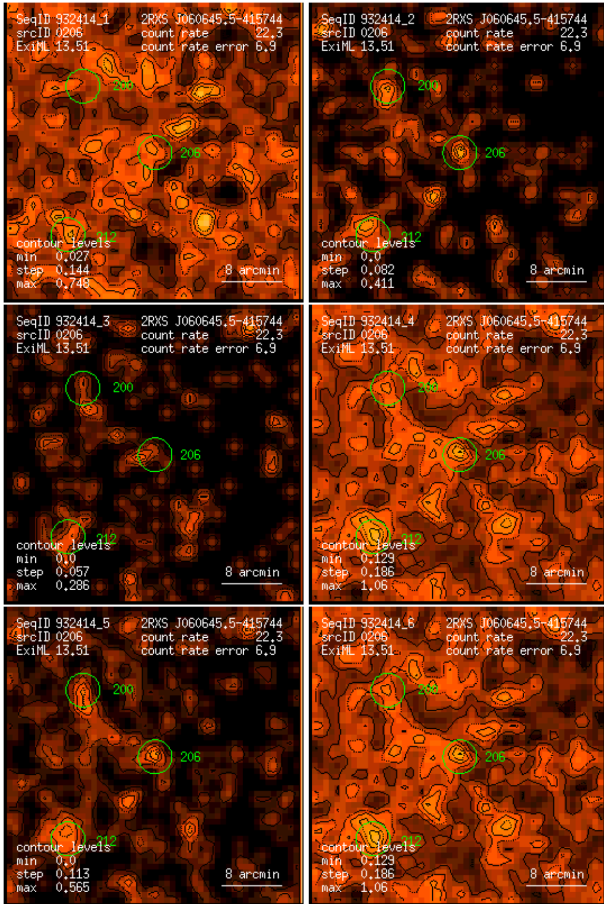
Figure 206: RASS 932414: detection 0206: band rate images, Gaussian filter: (1) PSPC channels 11 – 41, (2) 52 – 90, (3) 91 – 201, (4) 11 – 235, (5) 52 – 201, (6) 11 – 201. Broad band rates in counts/ks. Band rate contour levels in counts/ks/arcmin 2 .
