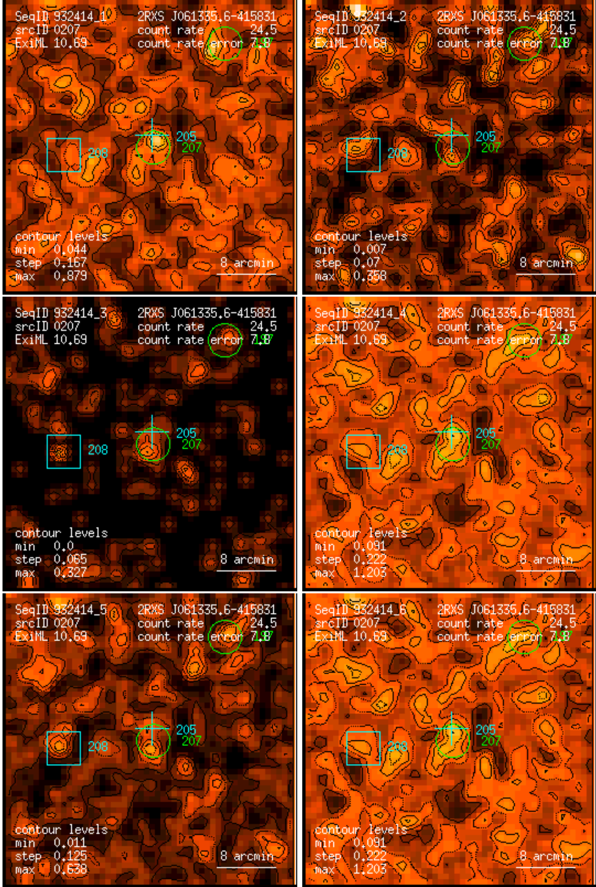
Figure 207: RASS 932414: detection 0207: band rate images, Gaussian filter: (1) PSPC channels 11 – 41, (2) 52 – 90, (3) 91 – 201, (4) 11 – 235, (5) 52 – 201, (6) 11 – 201. Broad band rates in counts/ks. Band rate contour levels in counts/ks/arcmin 2 .
