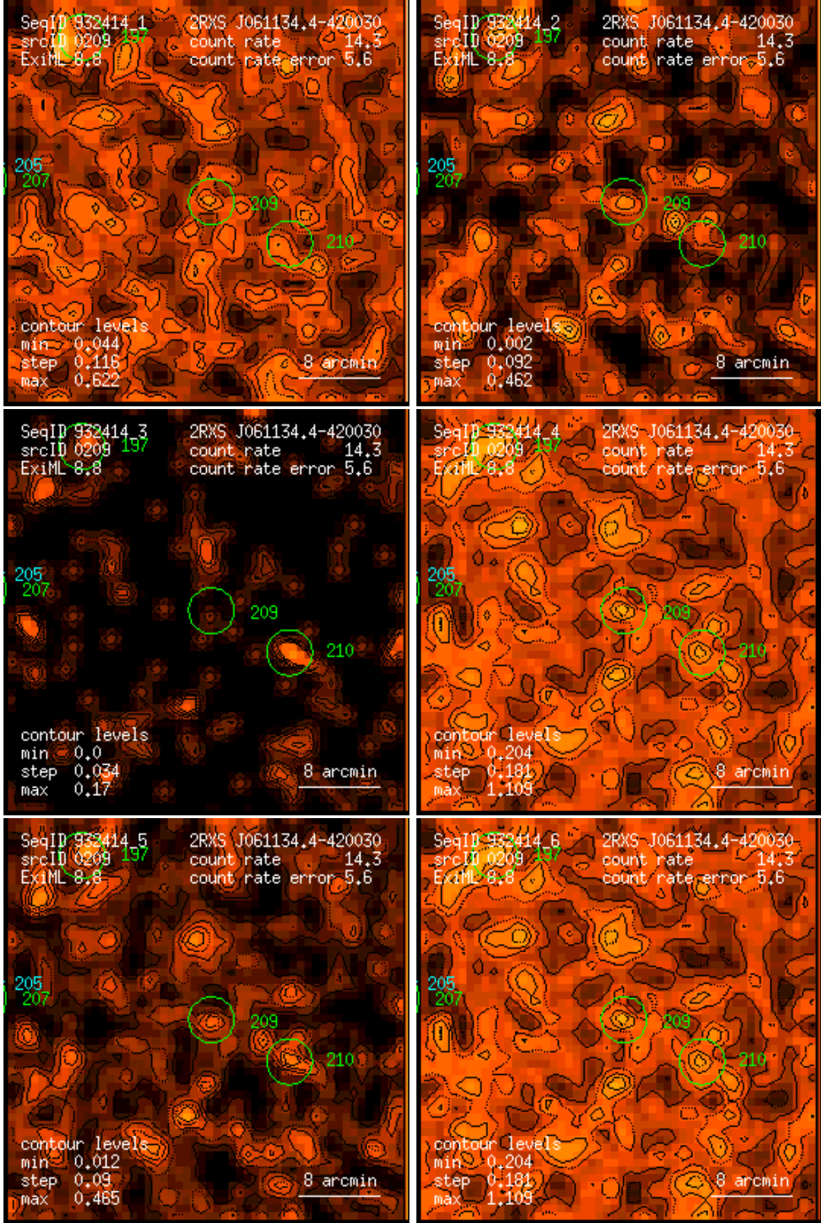
Figure 209: RASS 932414: detection 0209: band rate images, Gaussian filter: (1) PSPC channels 11 – 41, (2) 52 – 90, (3) 91 – 201, (4) 11 – 235, (5) 52 – 201, (6) 11 – 201. Broad band rates in counts/ks. Band rate contour levels in counts/ks/arcmin 2 .
