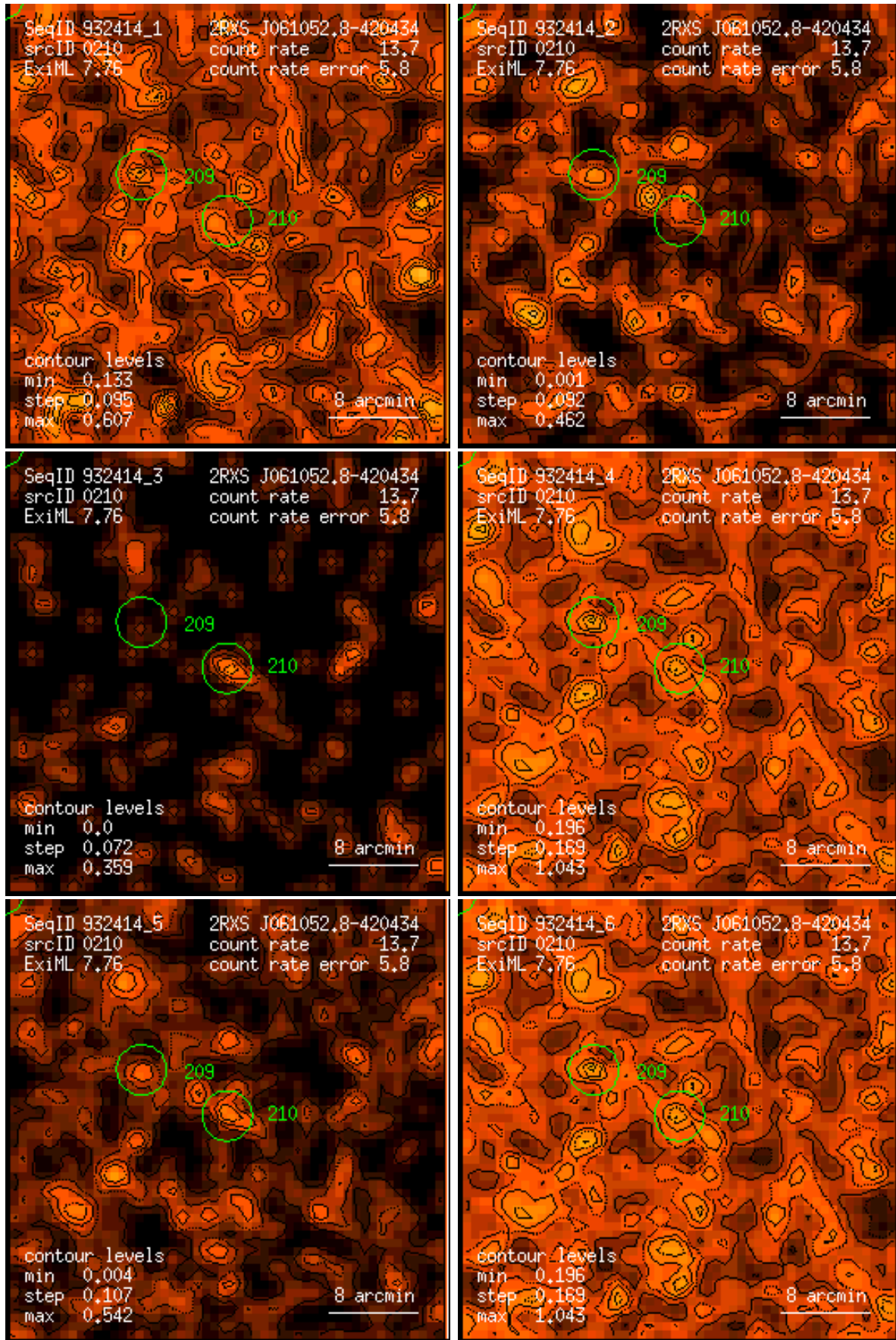
Figure 210: RASS 932414: detection 0210: band rate images, Gaussian filter: (1) PSPC channels 11 – 41, (2) 52 – 90, (3) 91 – 201, (4) 11 – 235, (5) 52 – 201, (6) 11 – 201. Broad band rates in counts/ks. Band rate contour levels in counts/ks/arcmin 2 .
