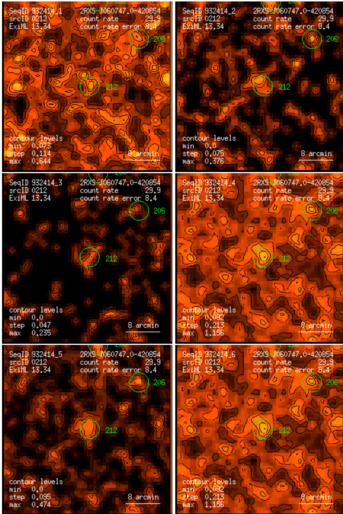
Figure 212: RASS 932414: detection 0212: band rate images, Gaussian filter: (1) PSPC channels 11 – 41, (2) 52 – 90, (3) 91 – 201, (4) 11 – 235, (5) 52 – 201, (6) 11 – 201. Broad band rates in counts/ks. Band rate contour levels in counts/ks/arcmin 2 .
