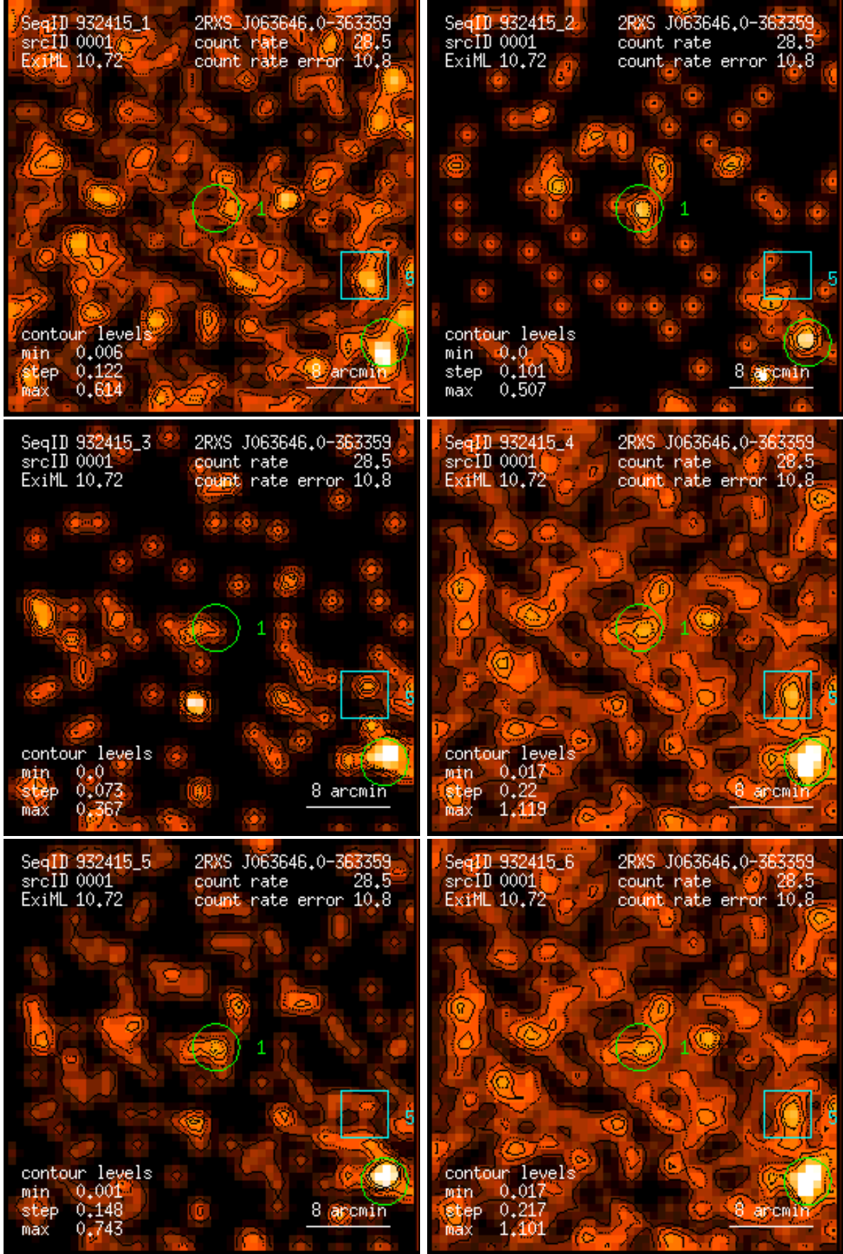
Figure 1: RASS 932415: detection 0001: band rate images, Gaussian filter: (1) PSPC channels 11 – 41, (2) 52 – 90, (3) 91 – 201, (4) 11 – 235, (5) 52 – 201, (6) 11 – 201. Broad band rates in counts/ks. Band rate contour levels in counts/ks/arcmin 2 .
