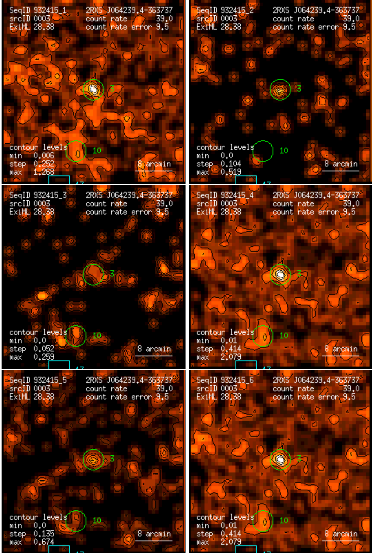
Figure 3: RASS 932415: detection 0003: band rate images, Gaussian filter: (1) PSPC channels 11 – 41, (2) 52 – 90, (3) 91 – 201, (4) 11 – 235, (5) 52 – 201, (6) 11 – 201. Broad band rates in counts/ks. Band rate contour levels in counts/ks/arcmin 2 .
