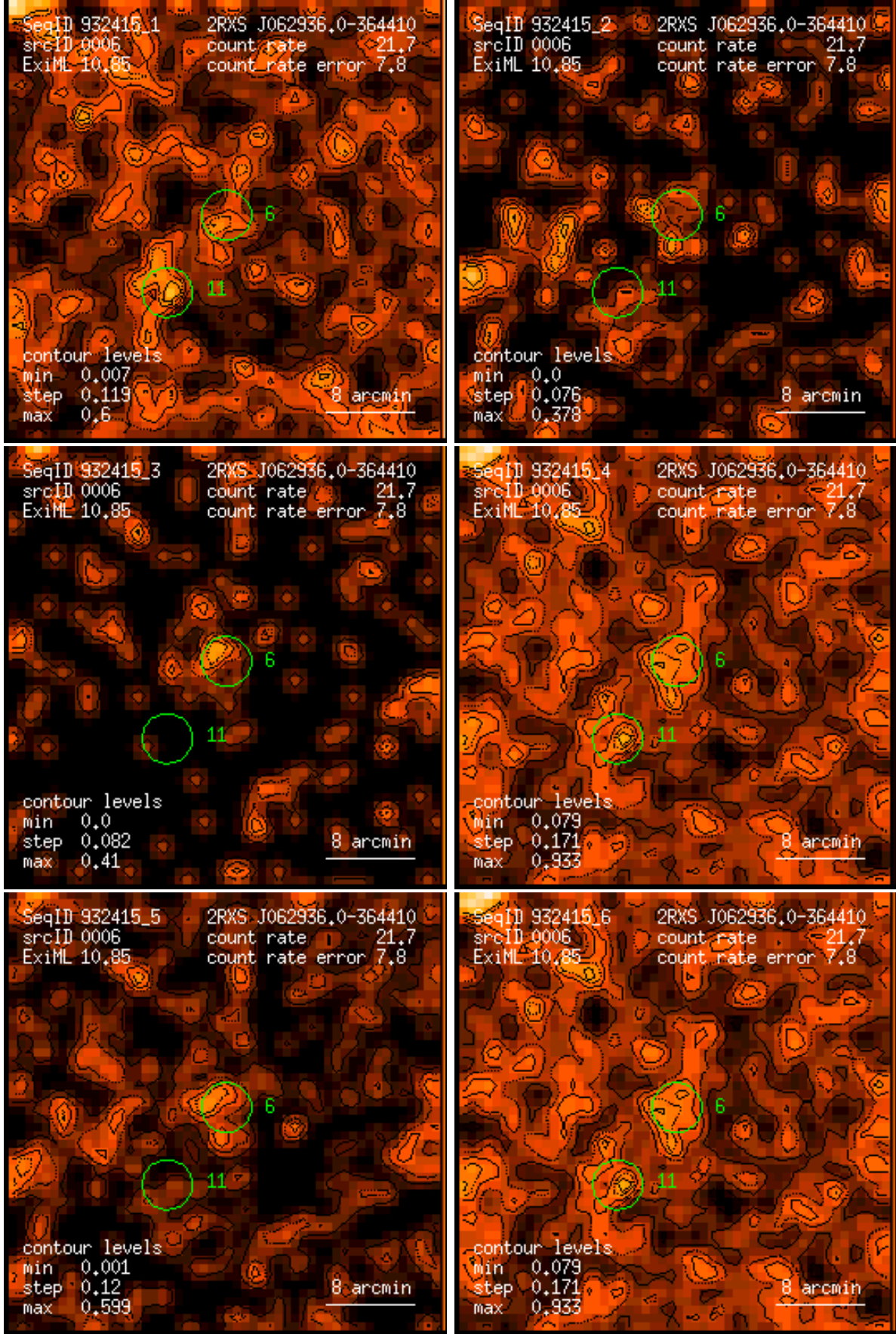
Figure 6: RASS 932415: detection 0006: band rate images, Gaussian filter: (1) PSPC channels 11 – 41, (2) 52 – 90, (3) 91 – 201, (4) 11 – 235, (5) 52 – 201, (6) 11 – 201. Broad band rates in counts/ks. Band rate contour levels in counts/ks/arcmin 2 .
