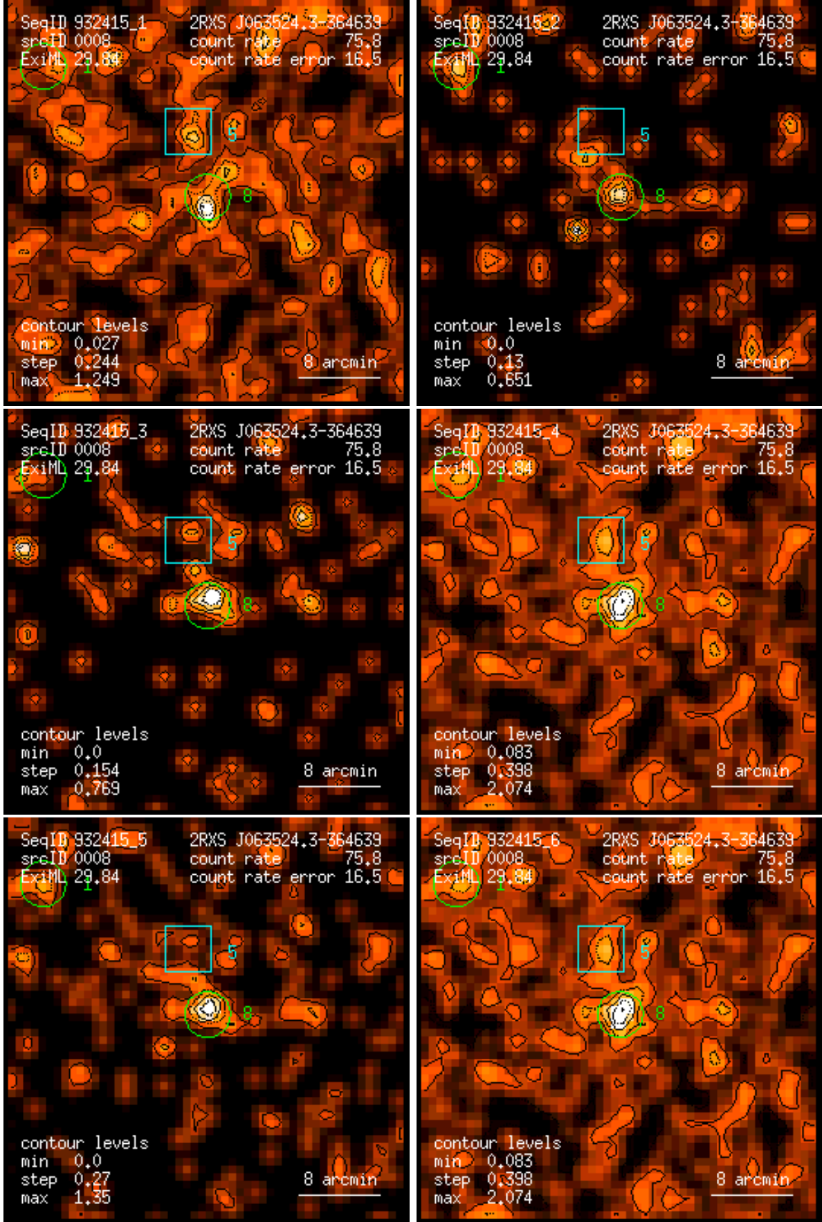
Figure 8: RASS 932415: detection 0008: band rate images, Gaussian filter: (1) PSPC channels 11 – 41, (2) 52 – 90, (3) 91 – 201, (4) 11 – 235, (5) 52 – 201, (6) 11 – 201. Broad band rates in counts/ks. Band rate contour levels in counts/ks/arcmin 2 .
