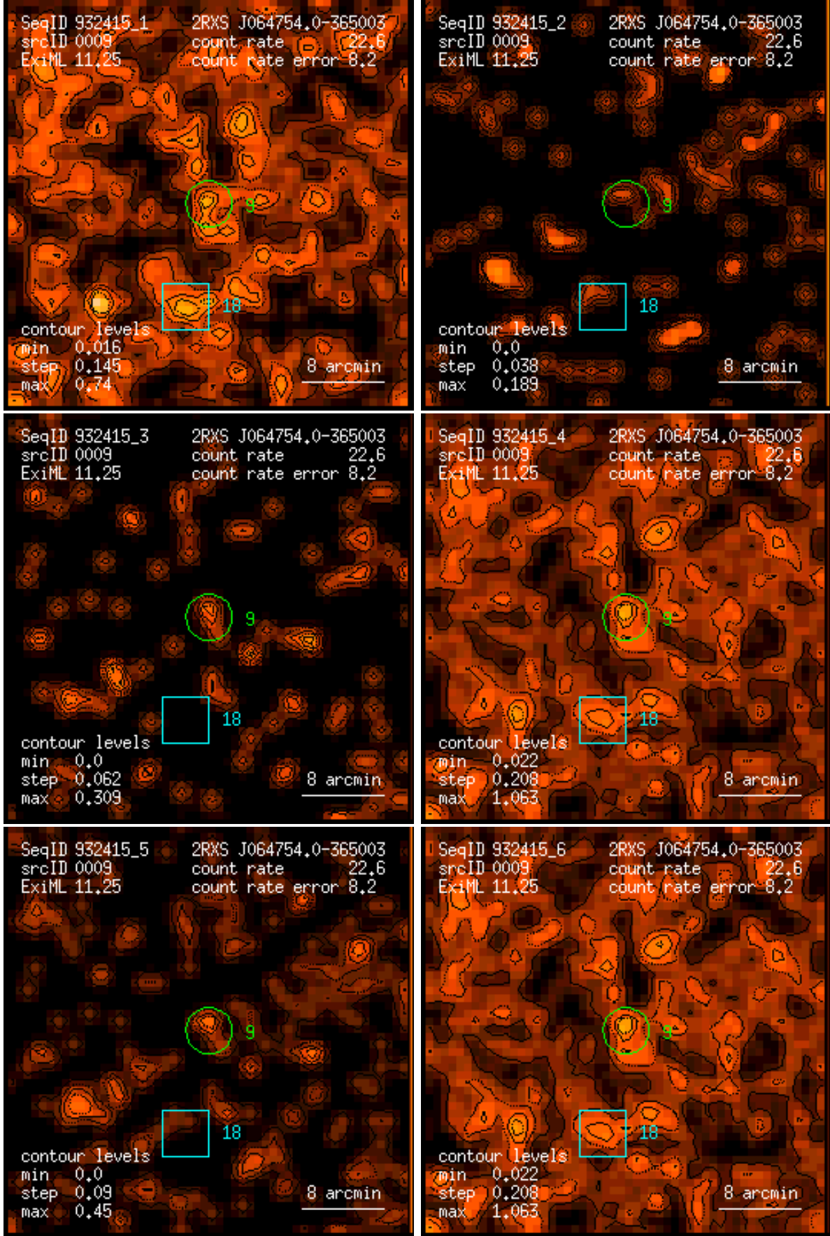
Figure 9: RASS 932415: detection 0009: band rate images, Gaussian filter: (1) PSPC channels 11 – 41, (2) 52 – 90, (3) 91 – 201, (4) 11 – 235, (5) 52 – 201, (6) 11 – 201. Broad band rates in counts/ks. Band rate contour levels in counts/ks/arcmin 2 .
