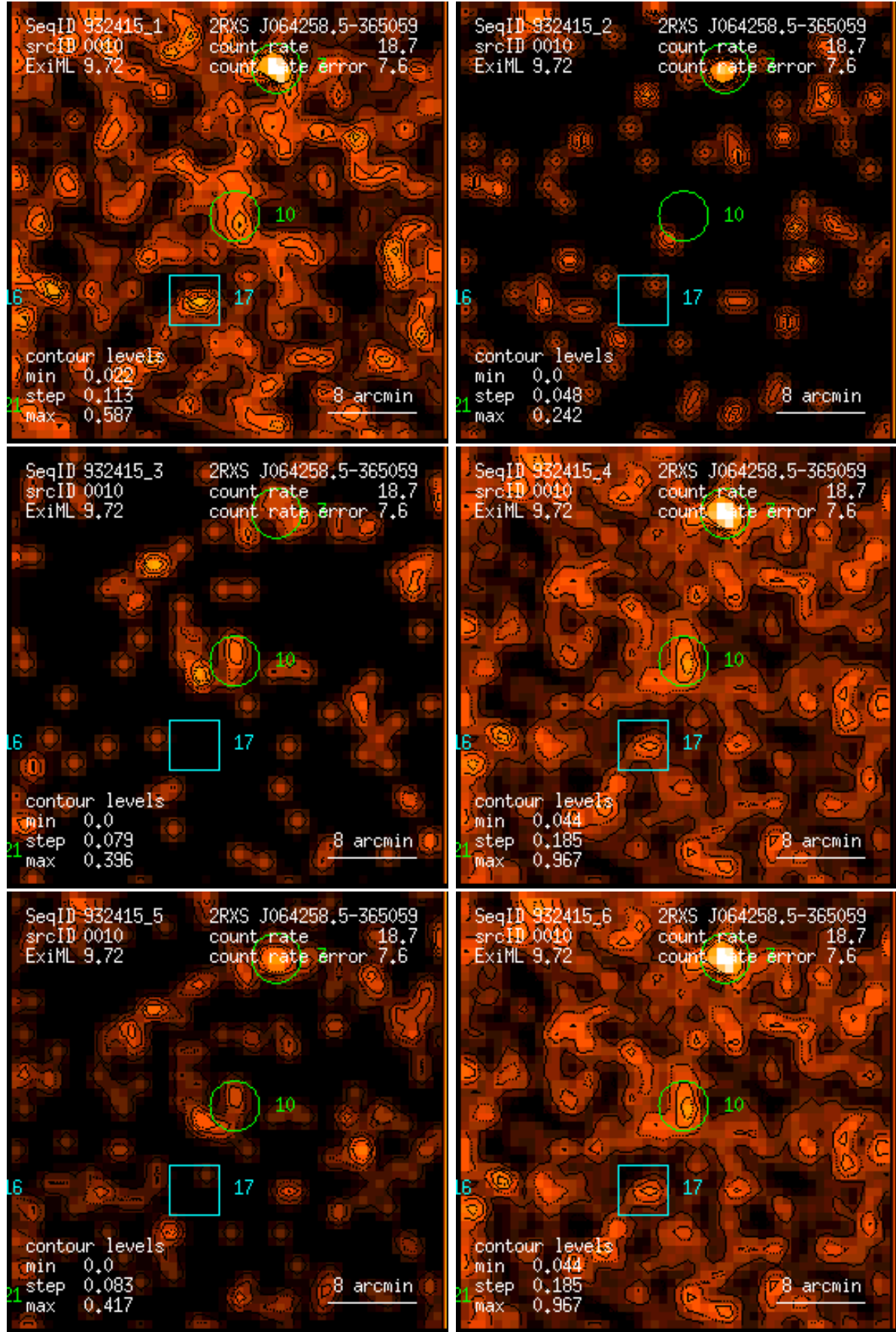
Figure 10: RASS 932415: detection 0010: band rate images, Gaussian filter: (1) PSPC channels 11 – 41, (2) 52 – 90, (3) 91 – 201, (4) 11 – 235, (5) 52 – 201, (6) 11 – 201. Broad band rates in counts/ks. Band rate contour levels in counts/ks/arcmin 2 .
