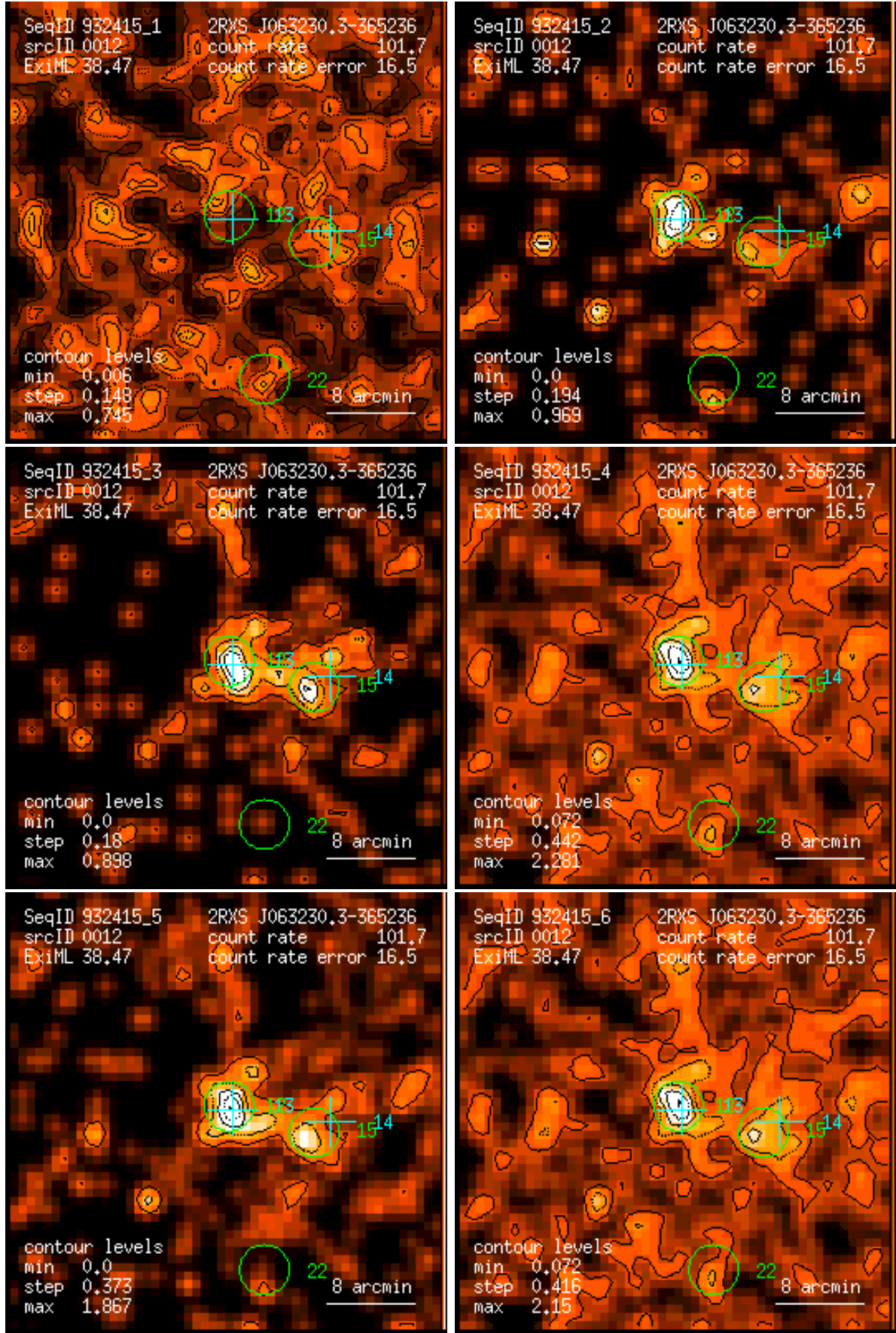
Figure 12: RASS 932415: detection 0012: band rate images, Gaussian filter: (1) PSPC channels 11 – 41, (2) 52 – 90, (3) 91 – 201, (4) 11 – 235, (5) 52 – 201, (6) 11 – 201. Broad band rates in counts/ks. Band rate contour levels in counts/ks/arcmin 2 .
