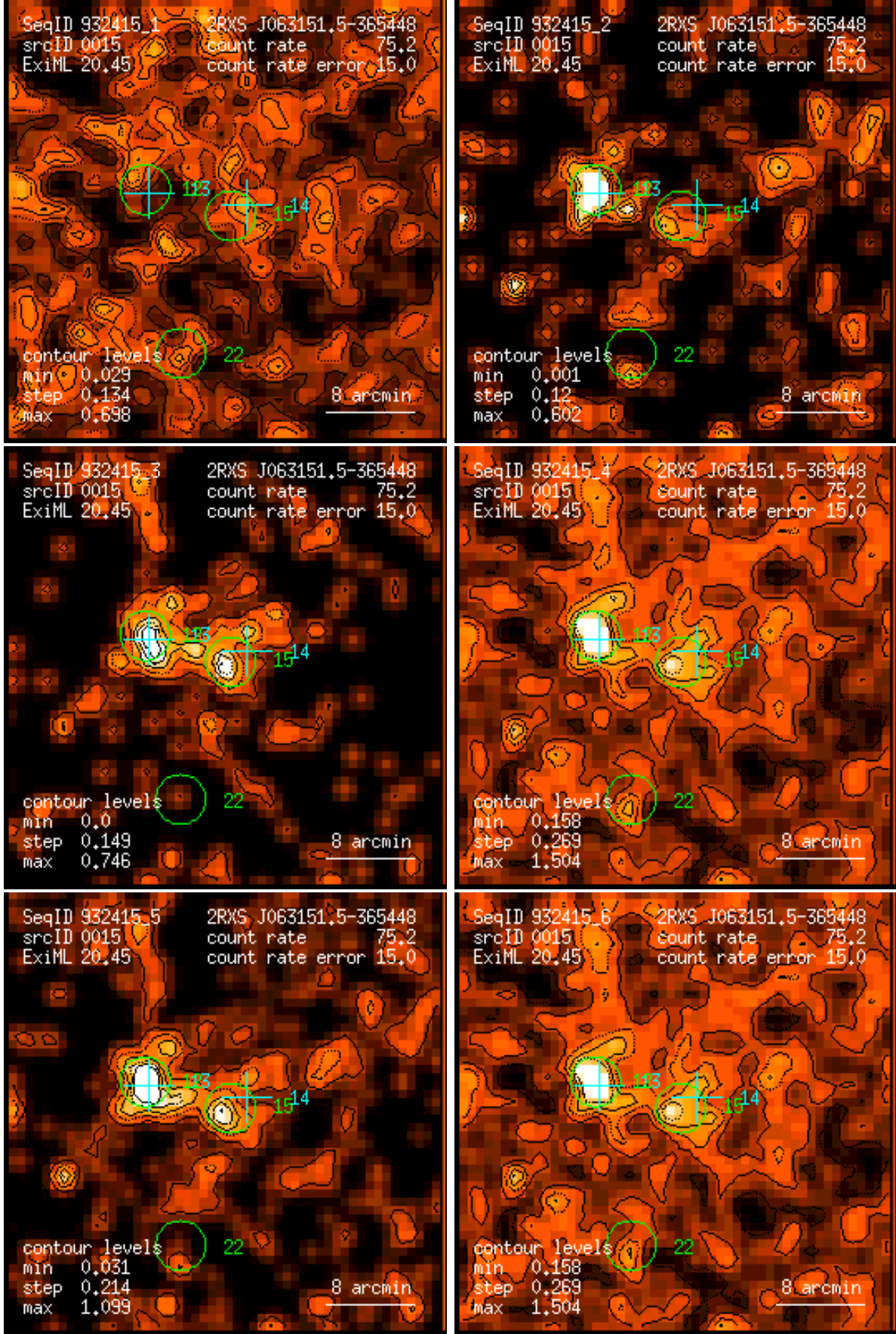
Figure 15: RASS 932415: detection 0015: band rate images, Gaussian filter: (1) PSPC channels 11 – 41, (2) 52 – 90, (3) 91 – 201, (4) 11 – 235, (5) 52 – 201, (6) 11 – 201. Broad band rates in counts/ks. Band rate contour levels in counts/ks/arcmin 2 .
