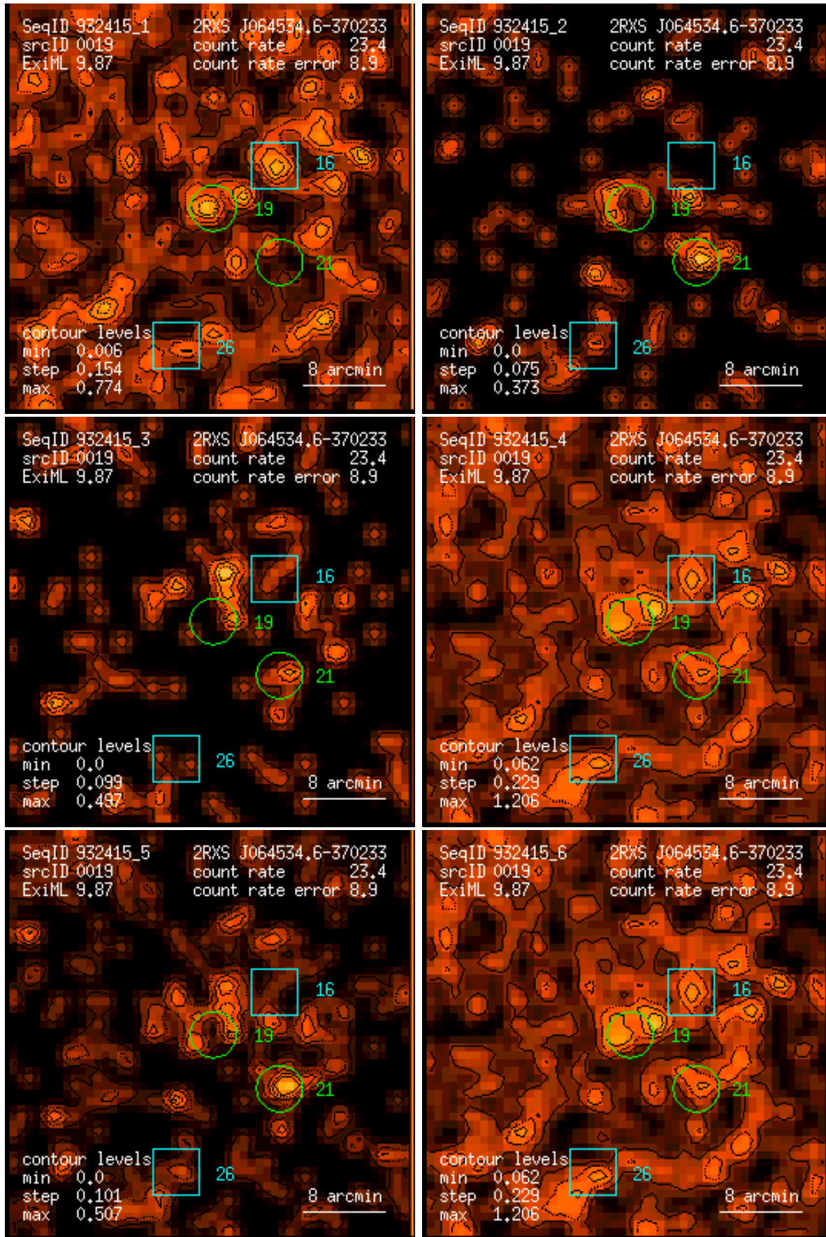
Figure 19: RASS 932415: detection 0019: band rate images, Gaussian filter: (1) PSPC channels 11 – 41, (2) 52 – 90, (3) 91 – 201, (4) 11 – 235, (5) 52 – 201, (6) 11 – 201. Broad band rates in counts/ks. Band rate contour levels in counts/ks/arcmin 2 .
