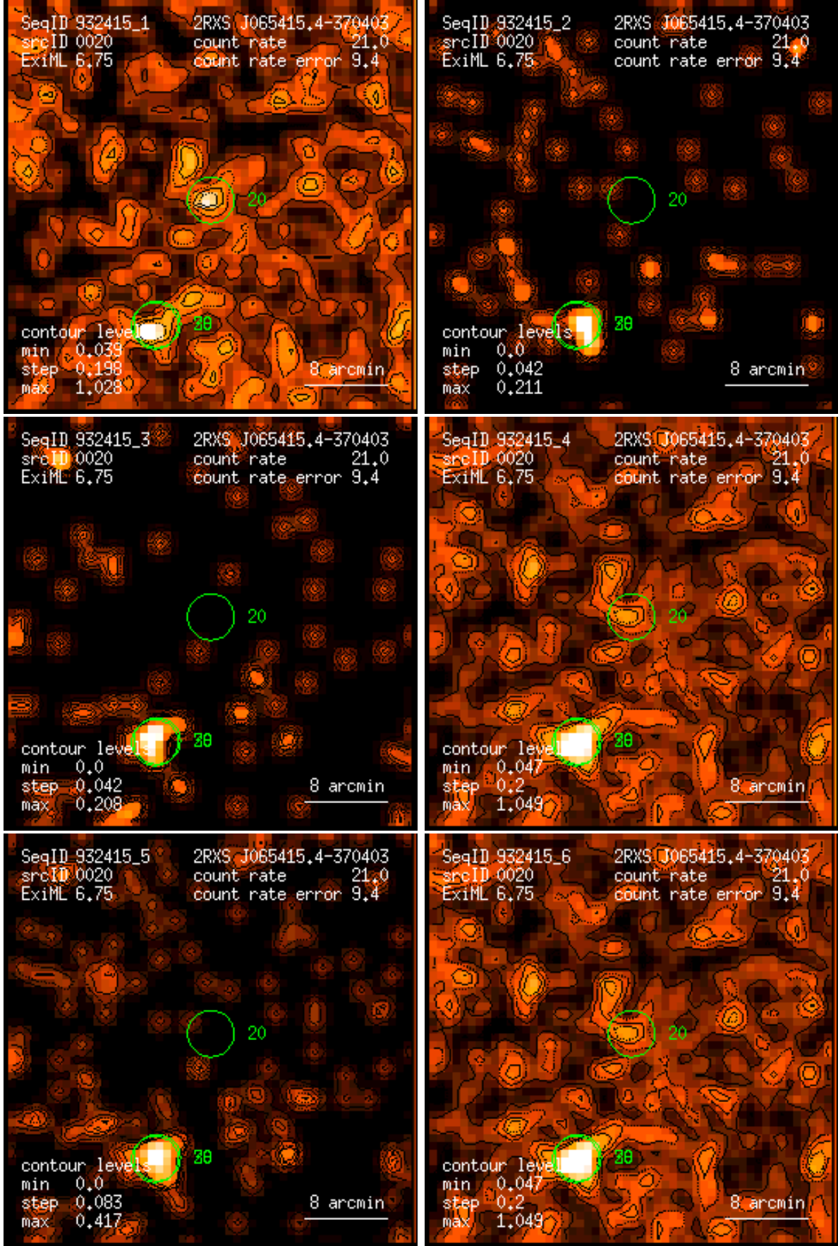
Figure 20: RASS 932415: detection 0020: band rate images, Gaussian filter: (1) PSPC channels 11 – 41, (2) 52 – 90, (3) 91 – 201, (4) 11 – 235, (5) 52 – 201, (6) 11 – 201. Broad band rates in counts/ks. Band rate contour levels in counts/ks/arcmin 2 .
