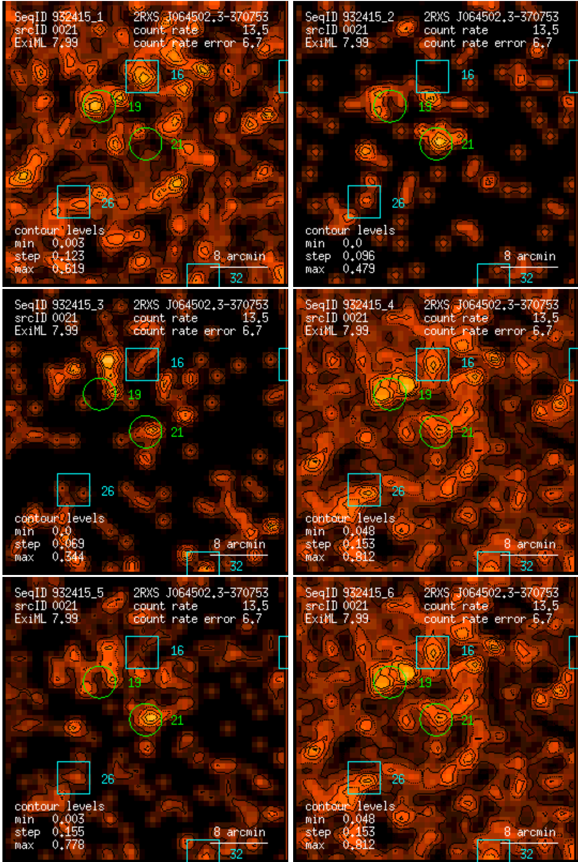
Figure 21: RASS 932415: detection 0021: band rate images, Gaussian filter: (1) PSPC channels 11 – 41, (2) 52 – 90, (3) 91 – 201, (4) 11 – 235, (5) 52 – 201, (6) 11 – 201. Broad band rates in counts/ks. Band rate contour levels in counts/ks/arcmin 2 .
