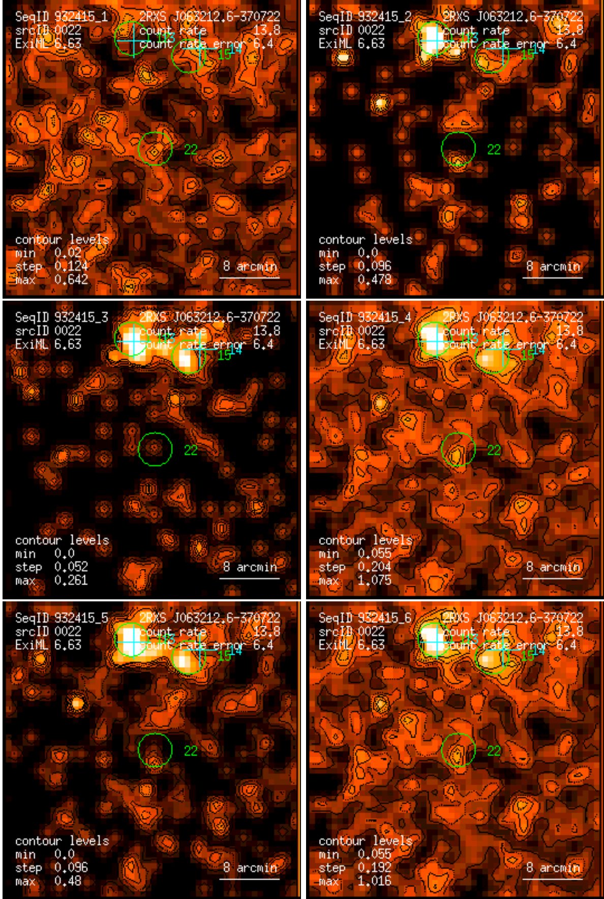
Figure 22: RASS 932415: detection 0022: band rate images, Gaussian filter: (1) PSPC channels 11 – 41, (2) 52 – 90, (3) 91 – 201, (4) 11 – 235, (5) 52 – 201, (6) 11 – 201. Broad band rates in counts/ks. Band rate contour levels in counts/ks/arcmin 2 .
