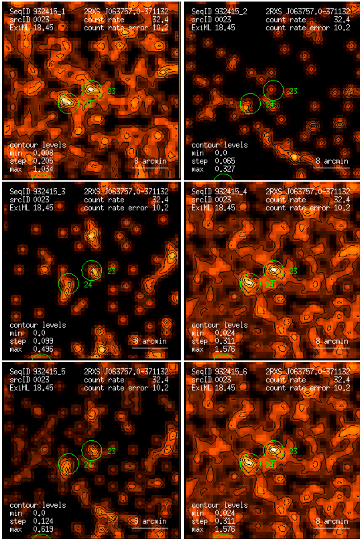
Figure 23: RASS 932415: detection 0023: band rate images, Gaussian filter: (1) PSPC channels 11 – 41, (2) 52 – 90, (3) 91 – 201, (4) 11 – 235, (5) 52 – 201, (6) 11 – 201. Broad band rates in counts/ks. Band rate contour levels in counts/ks/arcmin 2 .
