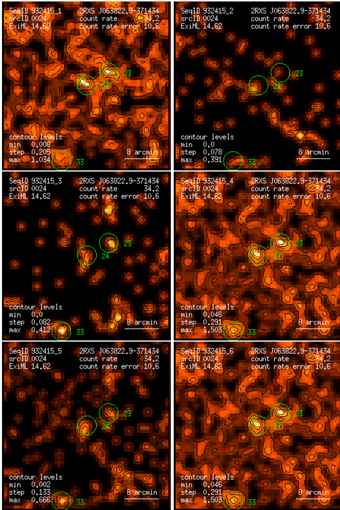
Figure 24: RASS 932415: detection 0024: band rate images, Gaussian filter: (1) PSPC channels 11 – 41, (2) 52 – 90, (3) 91 – 201, (4) 11 – 235, (5) 52 – 201, (6) 11 – 201. Broad band rates in counts/ks. Band rate contour levels in counts/ks/arcmin 2 .
