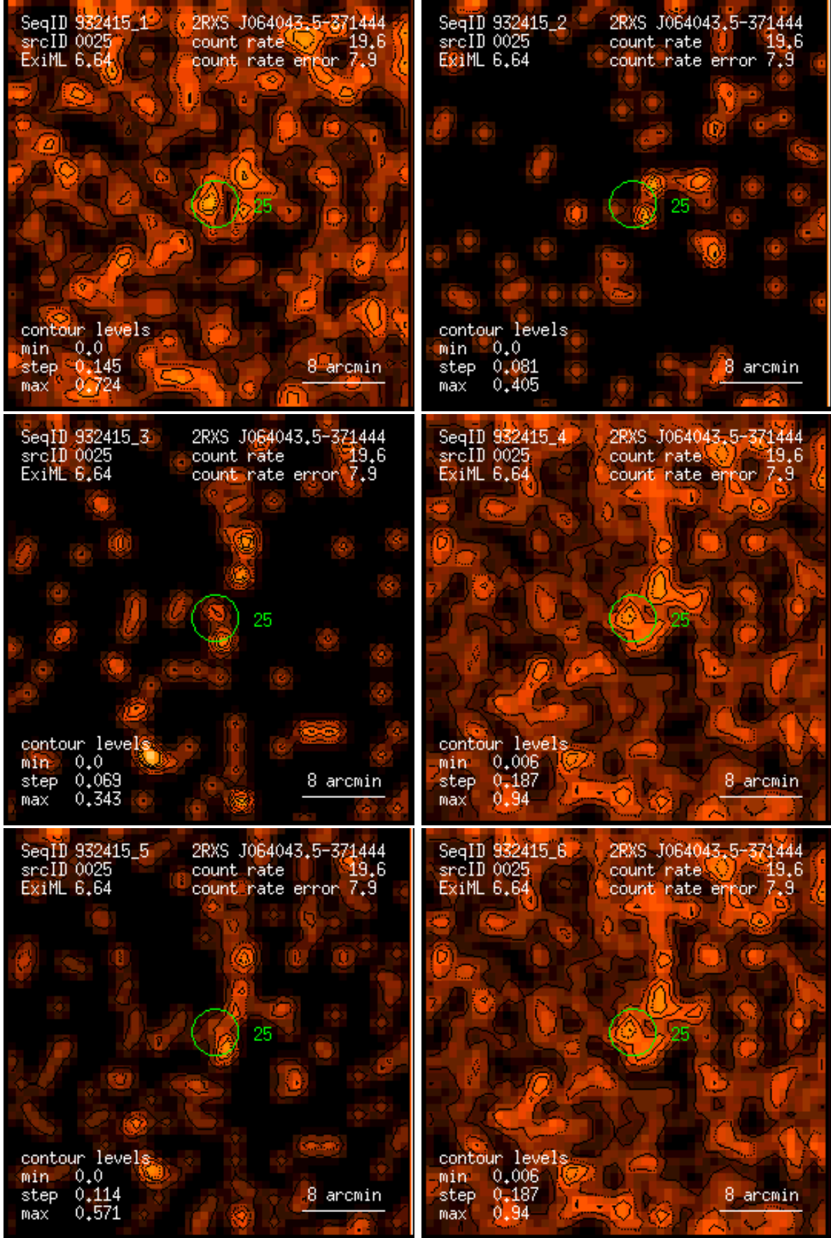
Figure 25: RASS 932415: detection 0025: band rate images, Gaussian filter: (1) PSPC channels 11 – 41, (2) 52 – 90, (3) 91 – 201, (4) 11 – 235, (5) 52 – 201, (6) 11 – 201. Broad band rates in counts/ks. Band rate contour levels in counts/ks/arcmin 2 .
