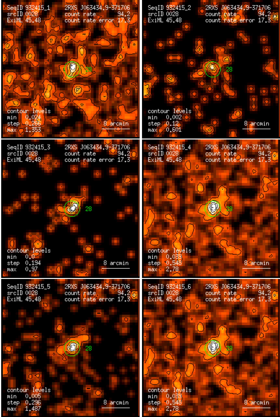
Figure 28: RASS 932415: detection 0028: band rate images, Gaussian filter: (1) PSPC channels 11 – 41, (2) 52 – 90, (3) 91 – 201, (4) 11 – 235, (5) 52 – 201, (6) 11 – 201. Broad band rates in counts/ks. Band rate contour levels in counts/ks/arcmin 2 .
