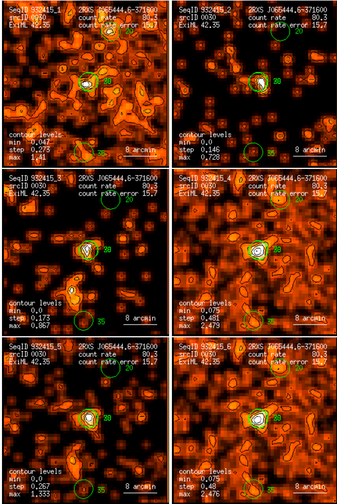
Figure 30: RASS 932415: detection 0030: band rate images, Gaussian filter: (1) PSPC channels 11 – 41, (2) 52 – 90, (3) 91 – 201, (4) 11 – 235, (5) 52 – 201, (6) 11 – 201. Broad band rates in counts/ks. Band rate contour levels in counts/ks/arcmin 2 .
