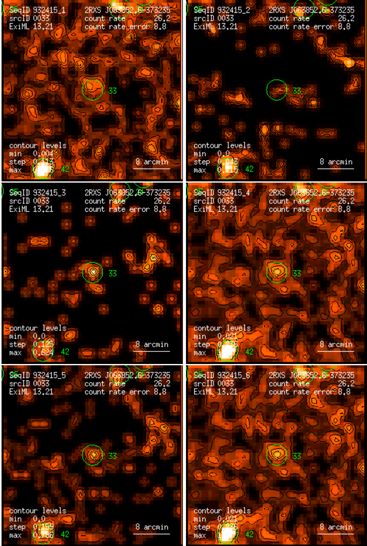
Figure 33: RASS 932415: detection 0033: band rate images, Gaussian filter: (1) PSPC channels 11 – 41, (2) 52 – 90, (3) 91 – 201, (4) 11 – 235, (5) 52 – 201, (6) 11 – 201. Broad band rates in counts/ks. Band rate contour levels in counts/ks/arcmin 2 .
