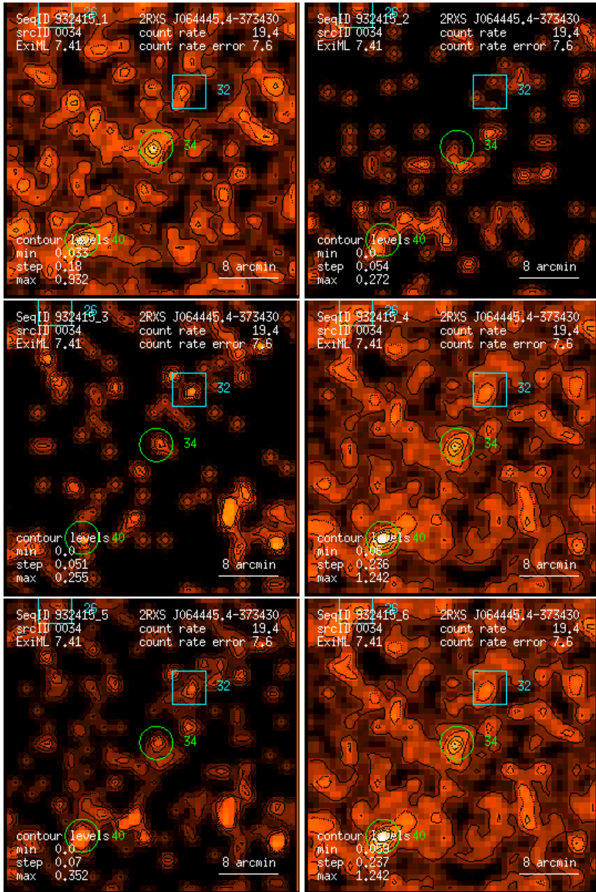
Figure 34: RASS 932415: detection 0034: band rate images, Gaussian filter: (1) PSPC channels 11 – 41, (2) 52 – 90, (3) 91 – 201, (4) 11 – 235, (5) 52 – 201, (6) 11 – 201. Broad band rates in counts/ks. Band rate contour levels in counts/ks/arcmin 2 .
