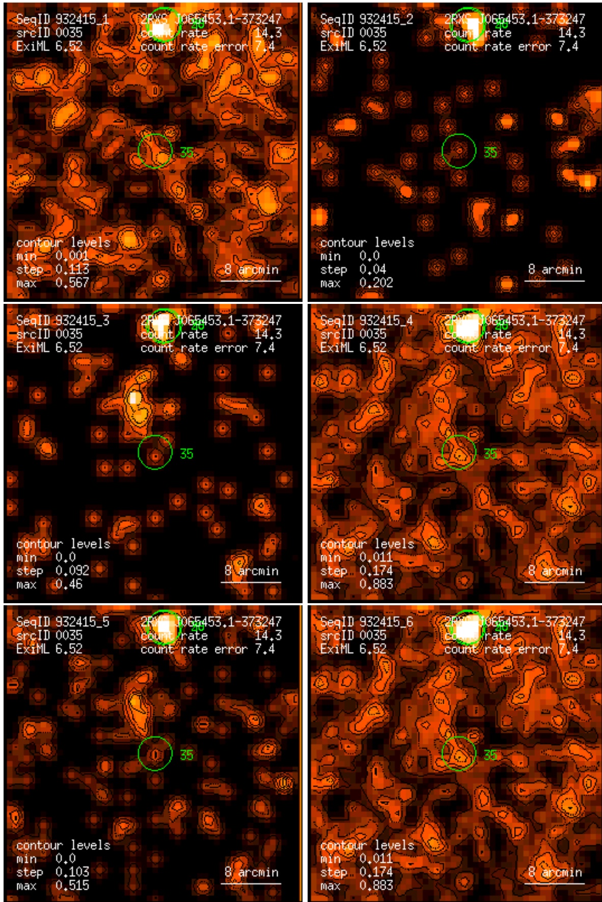
Figure 35: RASS 932415: detection 0035: band rate images, Gaussian filter: (1) PSPC channels 11 – 41, (2) 52 – 90, (3) 91 – 201, (4) 11 – 235, (5) 52 – 201, (6) 11 – 201. Broad band rates in counts/ks. Band rate contour levels in counts/ks/arcmin 2 .
