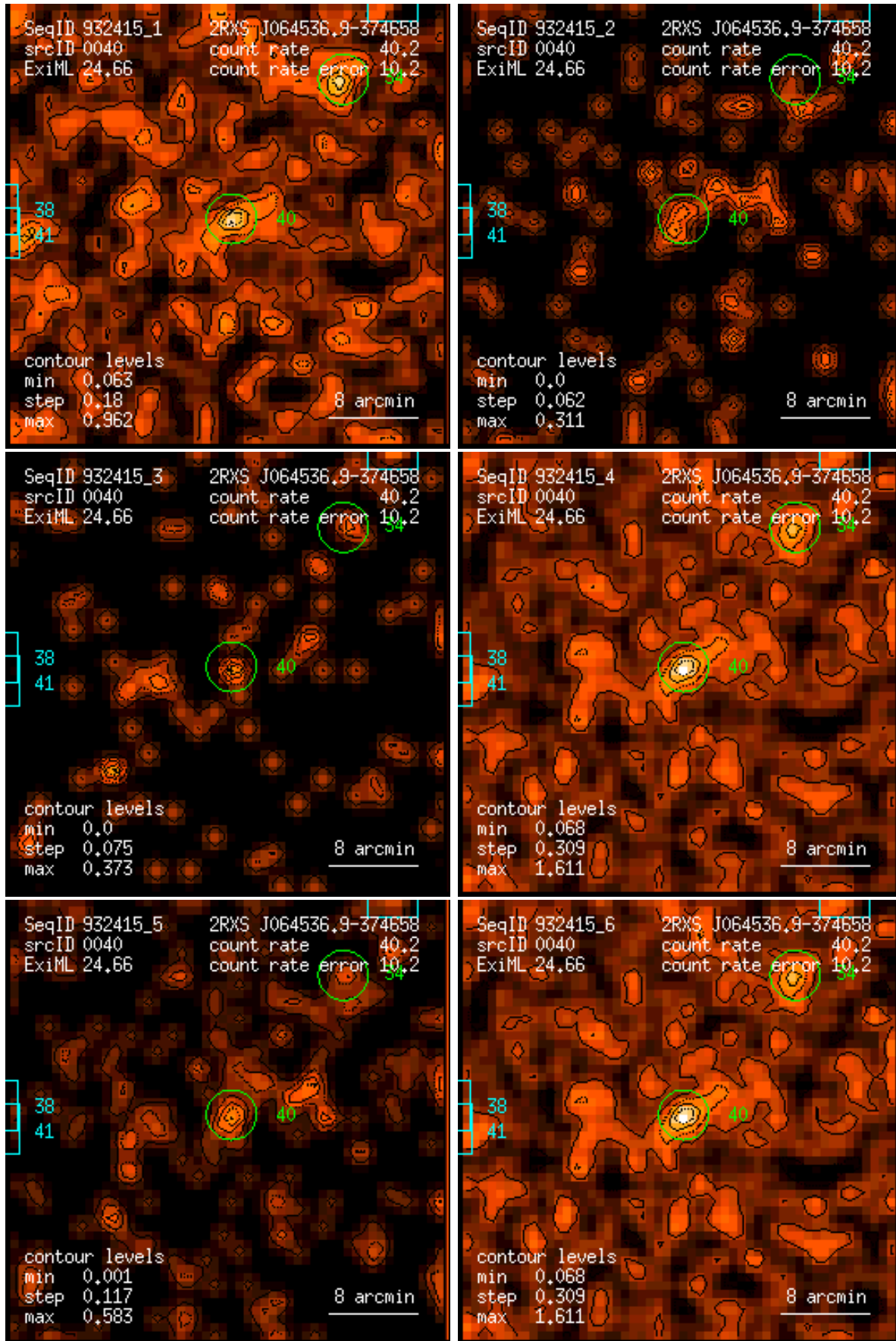
Figure 40: RASS 932415: detection 0040: band rate images, Gaussian filter: (1) PSPC channels 11 – 41, (2) 52 – 90, (3) 91 – 201, (4) 11 – 235, (5) 52 – 201, (6) 11 – 201. Broad band rates in counts/ks. Band rate contour levels in counts/ks/arcmin 2 .
