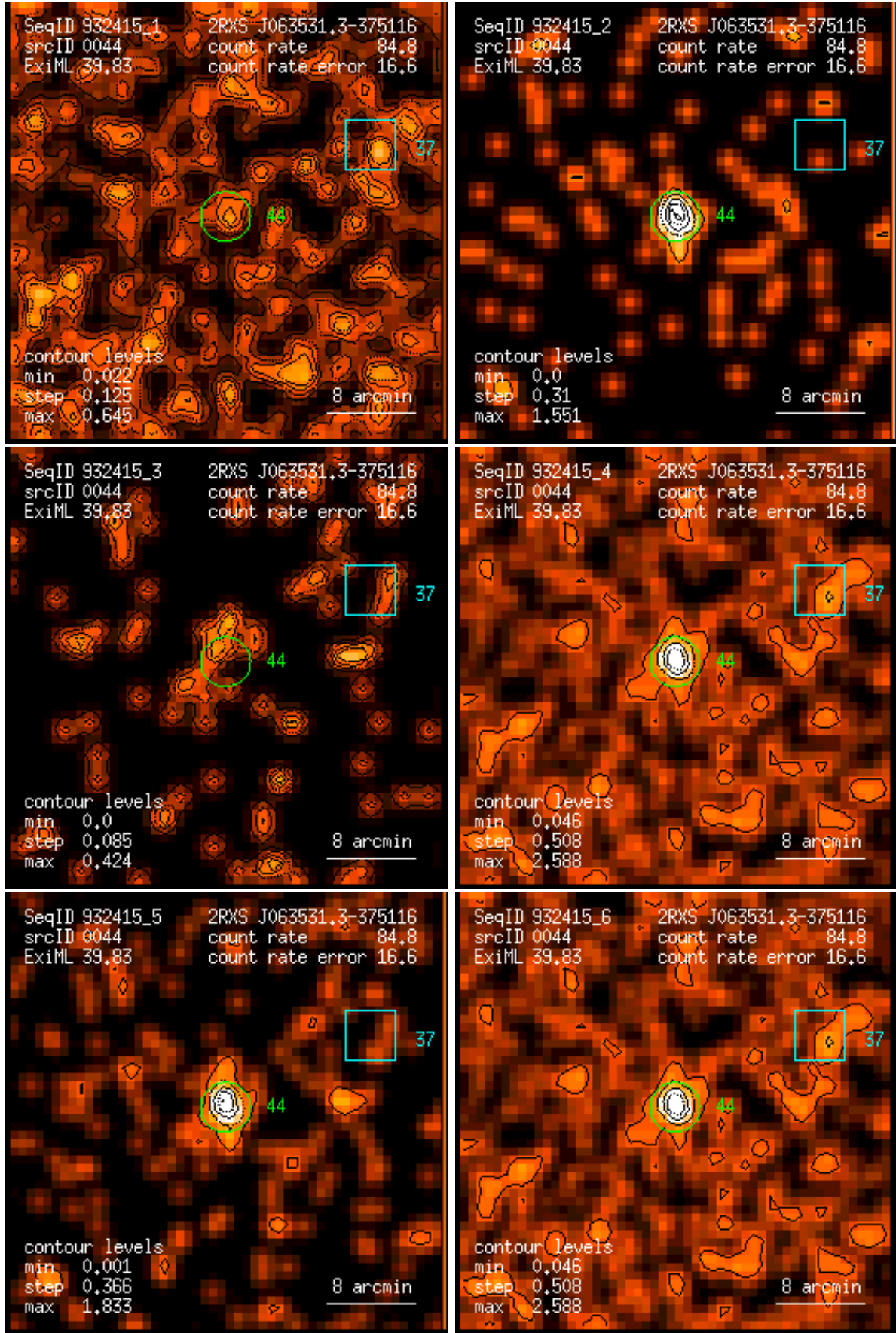
Figure 44: RASS 932415: detection 0044: band rate images, Gaussian filter: (1) PSPC channels 11 – 41, (2) 52 – 90, (3) 91 – 201, (4) 11 – 235, (5) 52 – 201, (6) 11 – 201. Broad band rates in counts/ks. Band rate contour levels in counts/ks/arcmin 2 .
